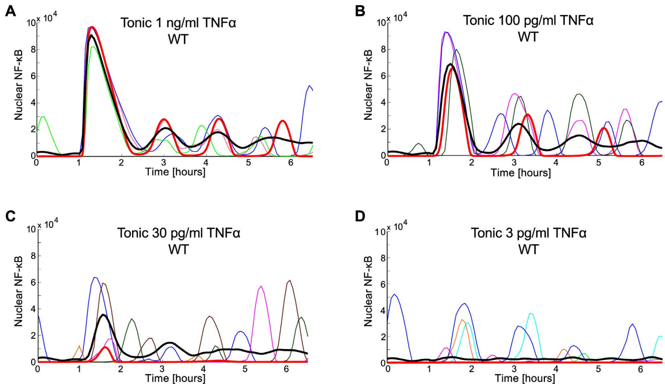
Figure 7. Simulated responses of WT cells (with \lambda=0.025 ) to tonic TNF \alpha stimulation beginning at t=1 h. (A–D): TNF \alpha doses: 1 ng/ml, 100 pg/ml, 30 pg/ml, 3 pg/ml. Red thick line – deterministic simulation; thin colored lines – single cell stochastic simulations; black thick line – population average. In (A) and (B), 3 individual representative cells trajectories are shown (in each panel). In (C) and (D), respectively 5 and 10 individual cell trajectories are shown, but only 3 trajectories (in each panel) exhibit visible oscillations. doi:10.1371/journal.pone.0078887.g007
