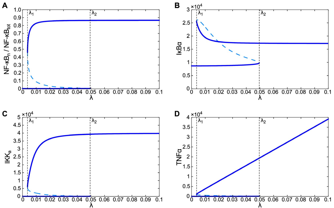
Figure 4. Bifurcation diagrams for A20-deficient cells. Stable recurrent solutions in a function of TNF \alpha mRNA transcription coefficient \lambda . (A–D) Nuclear NF- \kappa B, free cytoplasmic I \kappa B \alpha , active IKK, intracellular TNF \alpha . There are two saddle-node bifurcations at \lambda_1 and \lambda_2 . doi:10.1371/journal.pone.0078887.g004
