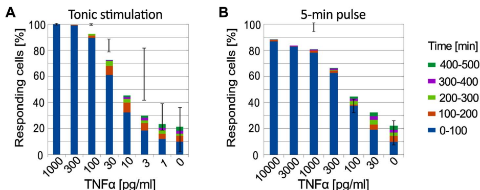
Figure 8. Fraction of responding cells versus TNF \alpha dose. (A) Tonic stimulation. (B) 5-min pulsed stimulation. Color bars: model prediction for \lambda=0.025 – fraction of cells responding within the given time period. Error bars show fractions of cells responding during the first 300-min in the experiment of Turner et al. [75] on SK-N-AS cells, see the main text. doi:10.1371/journal.pone.0078887.g008
