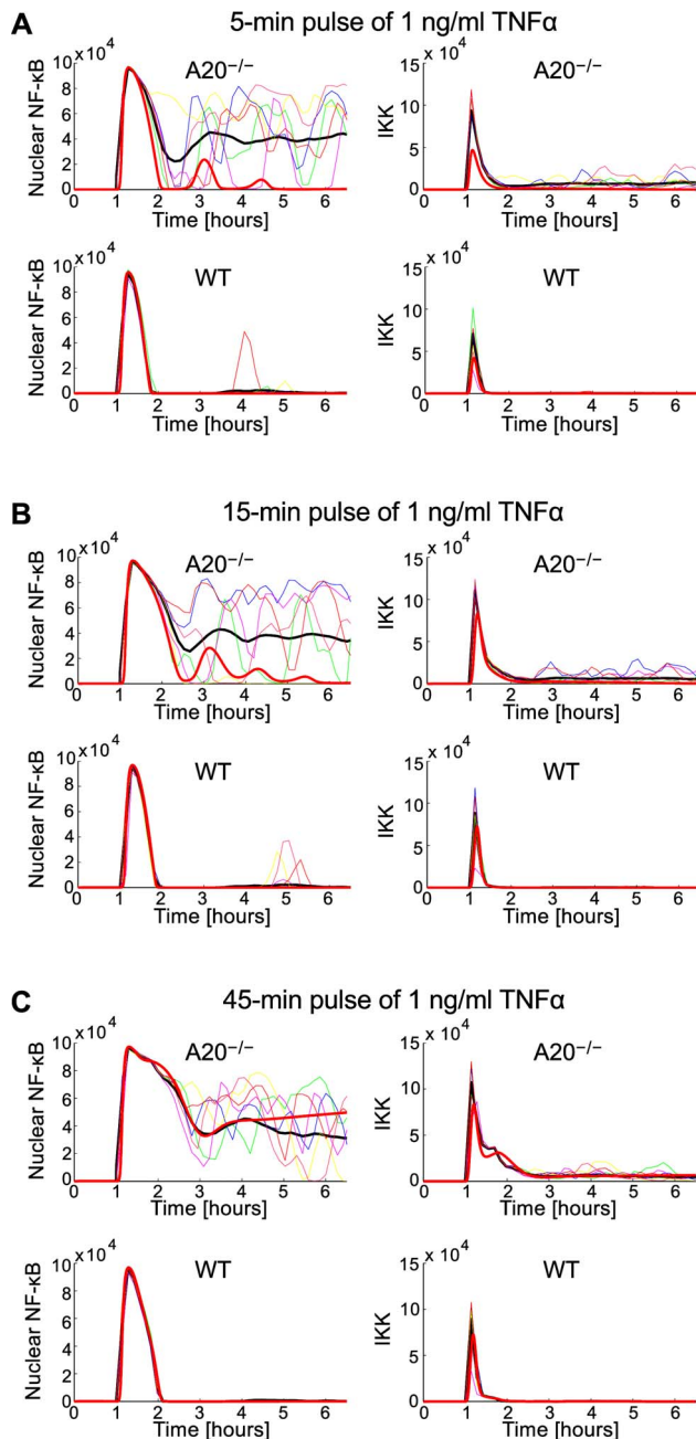
Figure 9. Simulated responses of WT and A20 -/- cells to pulsed stimulation with 1 ng/ml TNF \alpha for l=0.004 . (A) 5-min pulse. (B) 15-min pulse. (C) 45-min pulse. Red thick line – deterministic simulation; thin colored lines – single cell stochastic simulations; black thick line – population average. doi:10.1371/journal.pone.0078887.g009
