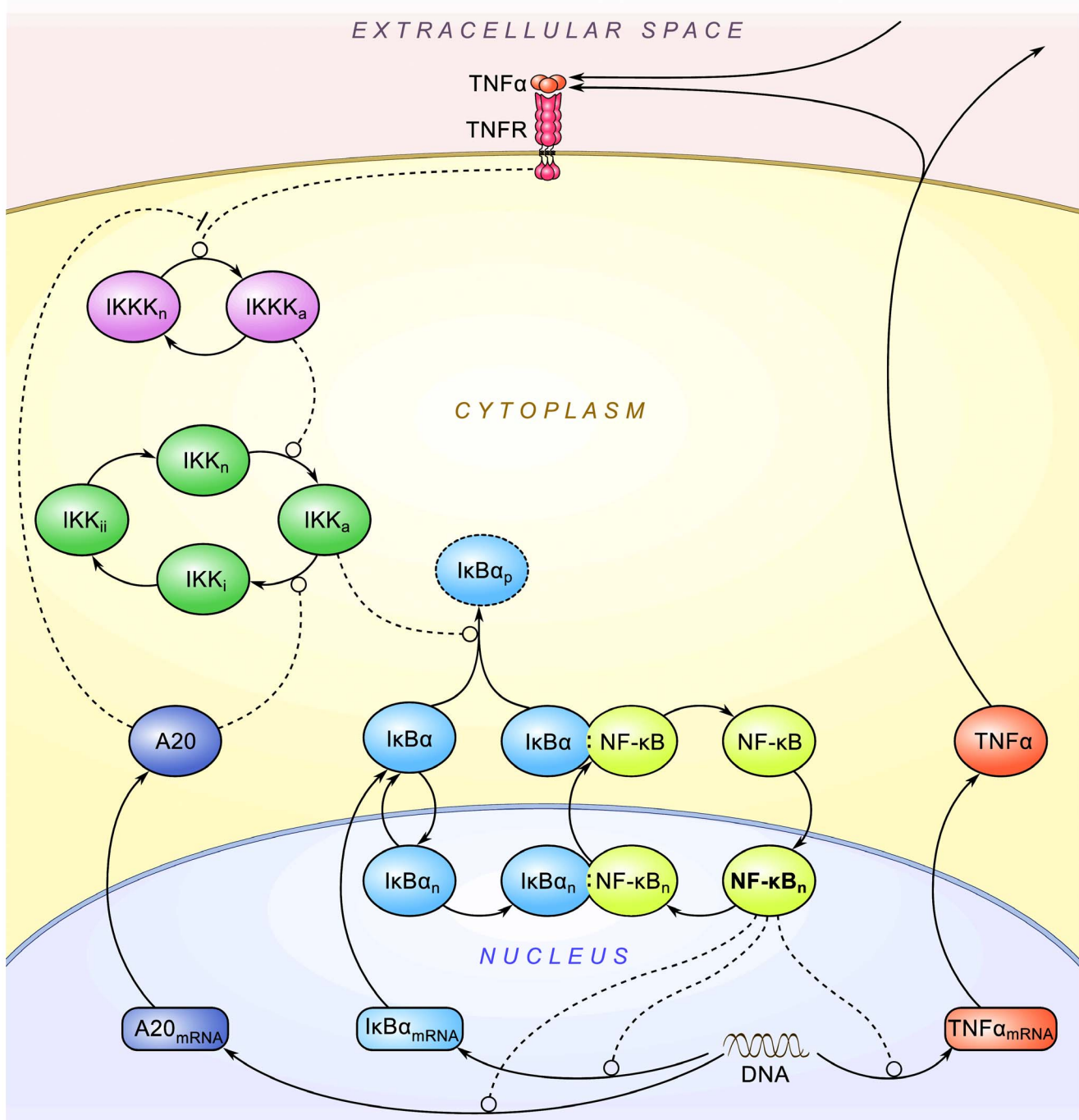
Figure 1. Schematic of the NF- \kappa B model. Solid arrow-headed lines denote transitions; dashed lines denote influence: positive for circle-headed lines, negative for hammer-headed lines. doi:10.1371/journal.pone.0078887.g001
