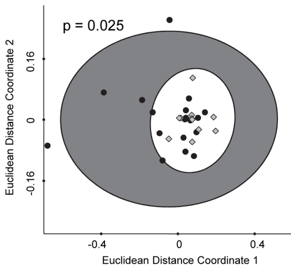
Figure 3. NMDS plot of Bd and non-Bd ponds according to pond physiochemistry. Ponds are ordinated according to Euclidian dissimilarities of standardized physiochemical variables (conductivity, pH, total nitrogen, total phosphorus, and chlorophyll-a). Bd ponds are light gray diamonds (encircled by the white 95% confidence ellipse) and non-Bd ponds are black circles (encircled by the dark 95% confidence ellipse). Ponds that are closer together are more similar to each other. Dispersion distance is significantly lower for the group of Bd ponds. doi:10.1371/journal.pone.0076035.g003
