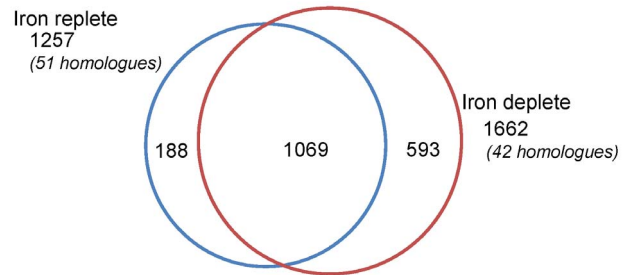
Figure 1. Venn diagram of number of proteins identified in Fe-replete and Fe-limited T. pseudonana . Proteins results presented were confidently identified from triplicate PAcIFIC analyses on the LTQ-VELOS. Fe-replete (blue) and Fe-limited (red) conditions were harvested at mid-exponential growth phase after acclimation. Numbers parenthetically annotated indicate homologous protein identifications. doi:10.1371/journal.pone.0075653.g001
