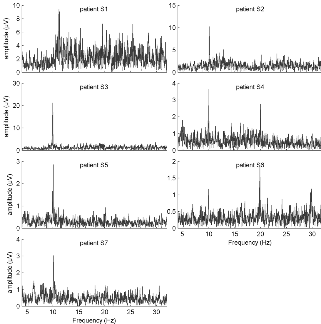
Figure 2. Results from the SSVEP scanning experiment: amplitude spectrum of the EEG response to the 10 Hz flickering square at electrode site O_2 for each patient. Note that for all patients, a peak at the stimulation frequency (and sometimes at its harmonic) can be observed in the amplitude spectrum.
