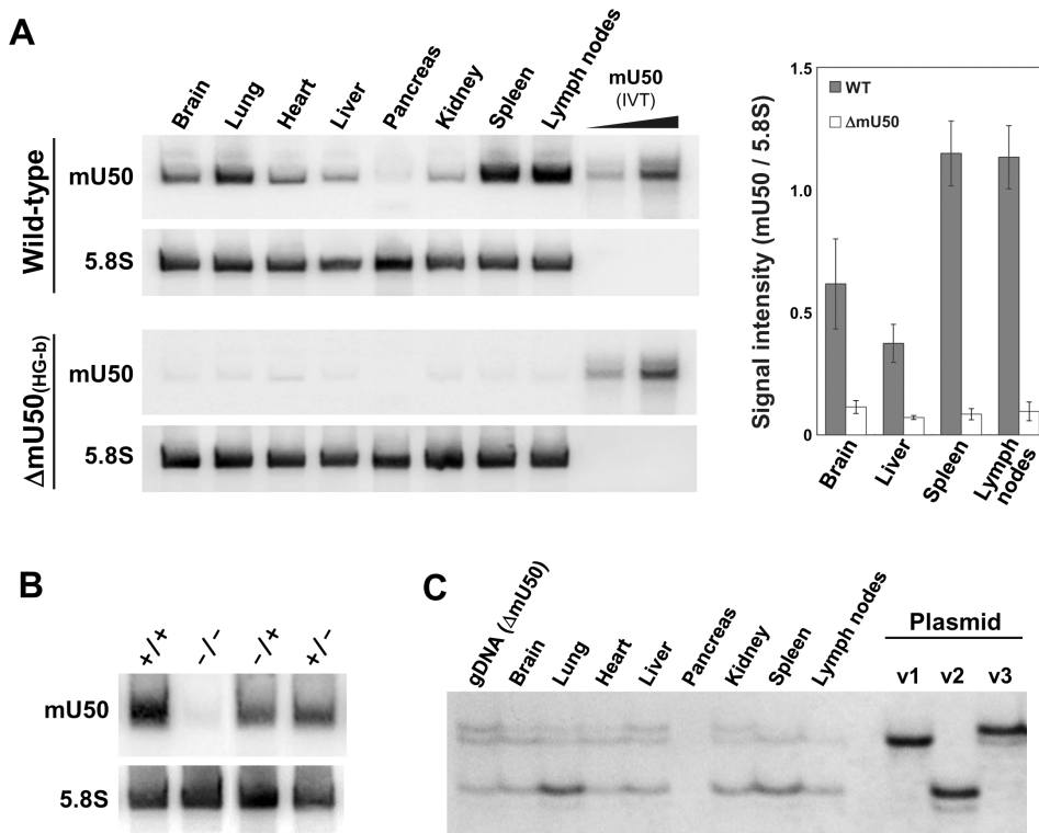
Figure 3. Molecular aspects of different organs in \Delta mU50_{(HG-b)} and wild-type mice. (A) Northern blot analysis of mU50 snoRNA expression in eight organs from wild-type and \Delta mU50_{(HG-b)} mice. In vitro transcribed (IVT) mU50 snoRNA was applied as a control. Detection of 5.8S rRNA was performed for the loading control. The signal intensities of selected organs are indicated in the panel on the right of the Figure. (B) Northern blot analysis of mU50 snoRNA and 5.8S rRNA expression in spleen obtained from wild-type (+/+), \Delta mU50_{(HG-b)} (-/-), and maternally (-/+) and paternally (+/-)-inherited \Delta mU50_{(HG-b)} heterozygotes. (C) PCR-SSCP analysis of the mU50 snoRNA variants in \Delta mU50_{(HG-b)} mice. Genomic DNA from \Delta mU50_{(HG-b)} mouse, which contains a single copy of each mU50HG-a paralog, was used as the control PCR template. gDNA: genomic DNA; v1, v2 and v3: plasmids that correspond to the mU50 snoRNAs encoded by mU50HG-a(1) , -a(2) , and -a(3) , respectively. doi:10.1371/journal.pone.0072105.g003
