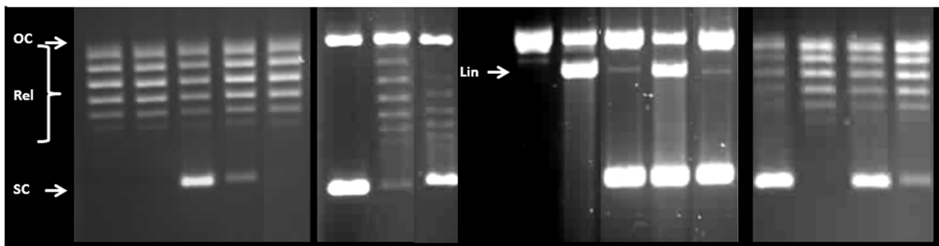
Figure 1. Evaluation of the activity of digested MccB17 mixtures. Effect of the alkaline hydrolysate (Hyd) of MccB17 on supercoiling (A), relaxation (B) and cleavage (C) assays with E. coli gyrase. The DNA species are annotated as follow: OC (open circular), Rel (relaxed), SC (supercoiled), and Lin (linear). Activity is compared with ciprofloxacin (CFX) and MccB17 (Mcc). (D) Effects of a mixture resulting from the digestion of MccB17 by subtilisin (Sub) in a supercoiling assay with E. coli gyrase compared to controls without inhibitors, and with ciprofloxacin (CFX) and MccB17 (Mcc). All reactions contain 3.3% DMSO.
