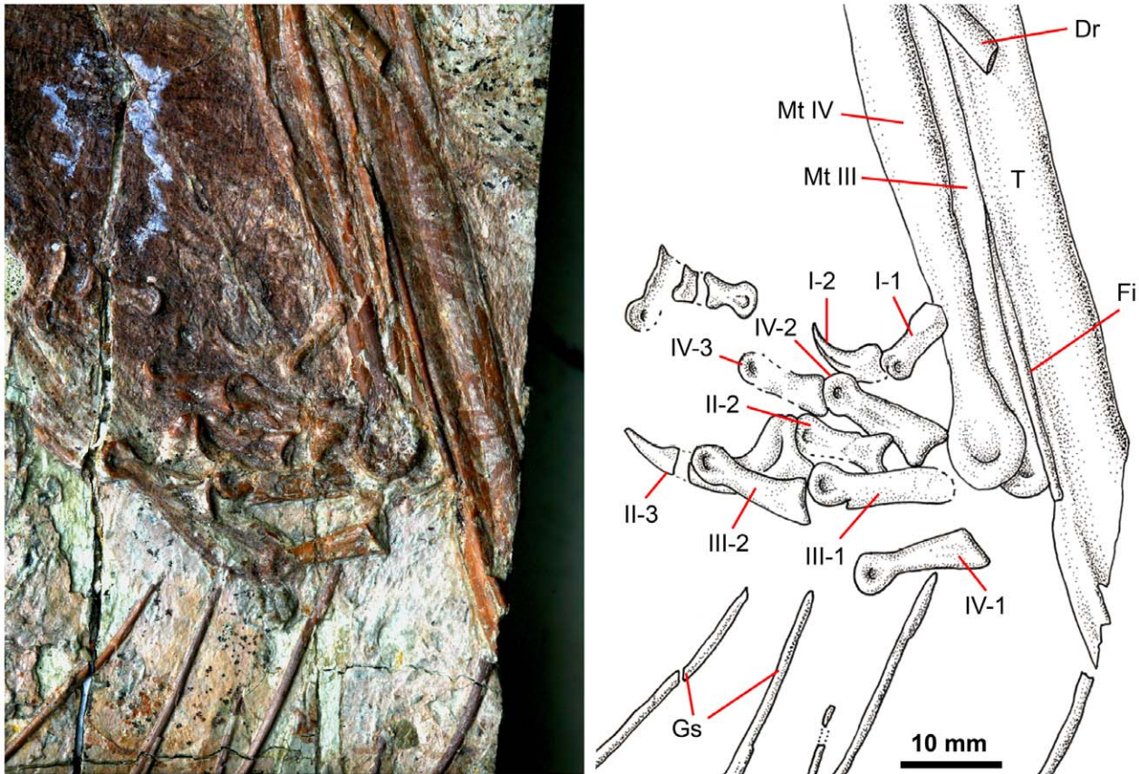
Figure 7. Close up of Sinornithosaurus right hindlimb within the abdominal cavity of Sinocallopteryx (JMP-V-05-8-01). Photograph and interpretive illustration. Gastralia (Gs) and dorsal rib (Dr) belong to Sinocallopteryx . Note the similar lengths of metatarsals III and IV. Abbreviations: Fi, fibula; Mt, metatarsal; T, tibia. doi:10.1371/journal.pone.0044012.g007
