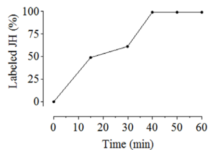
Figure 4. The efficiency of derivatization of the JH III epoxide ring with DBD-COCl. Fluorescence signal increases with time of incubation up to 40 minutes. Each point represents the percentage of tagged JH III peak area measured by HPLC-FD. Data represent the means \pm SD of three independent experiments. doi:10.1371/journal.pone.0043784.g004
