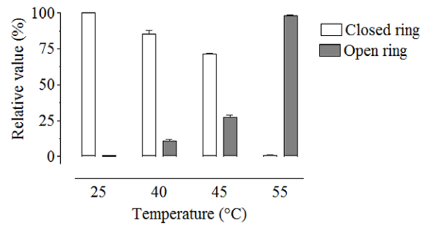
Figure 3. Effect of temperature on the opening of the epoxide ring of JH III. JH III was incubated with sodium sulphide (100 mM) at different temperatures. White bars indicate the percentage of intact JH III after the reaction and dark bars indicate JH III with open rings after the reaction. Data represent the means \pm SD of three independent experiments. doi:10.1371/journal.pone.0043784.g003
