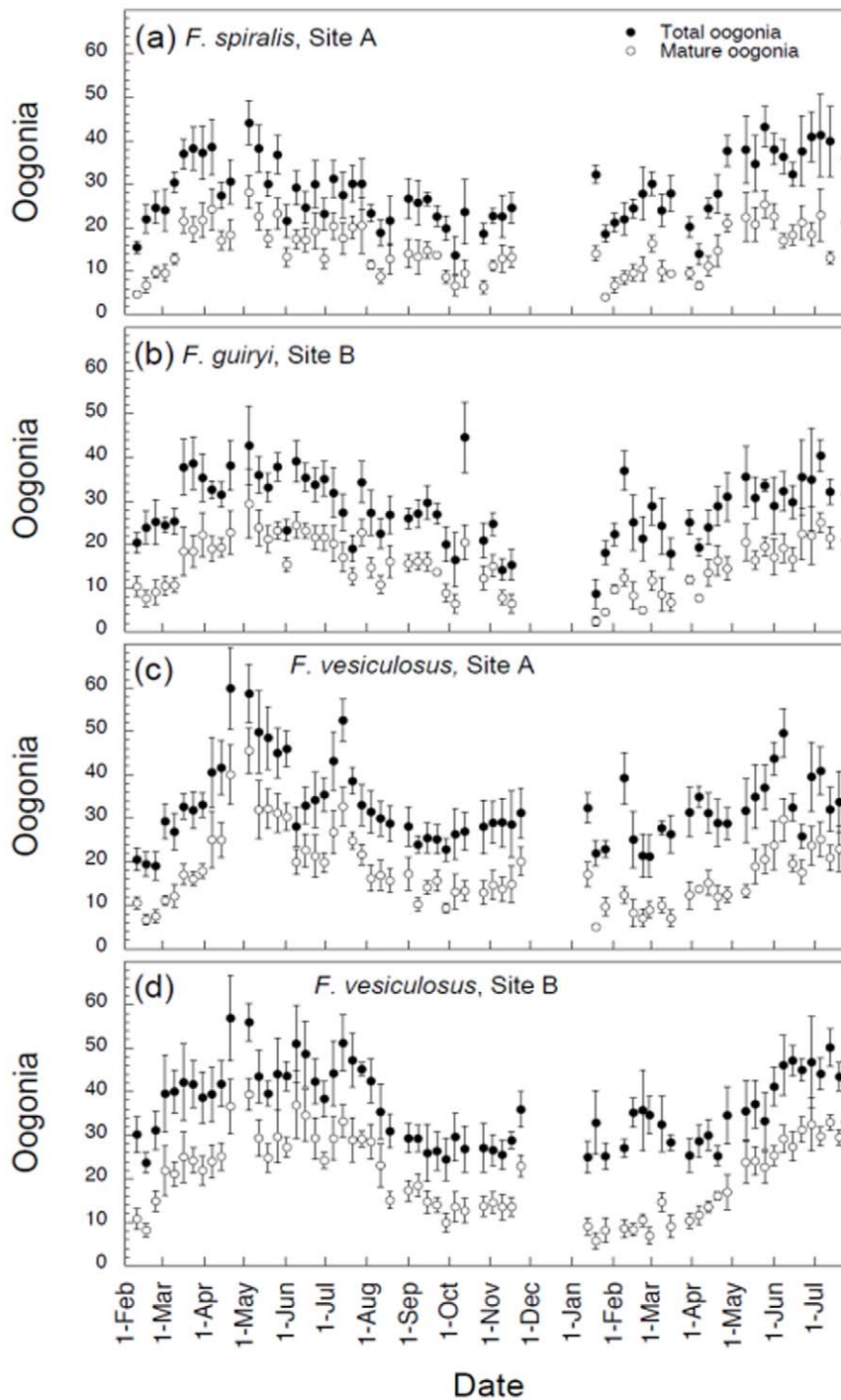
Figure 3. Total number of oogonia (closed symbols) and number of mature oogonia (open symbols) per conceptacle ( n=5 receptacles, \pm SE) from Fucus spiralis (plot a), Fucus guiryi (plot b), and Fucus vesiculosus (plots c and d) between February 2002 and July 2003.
