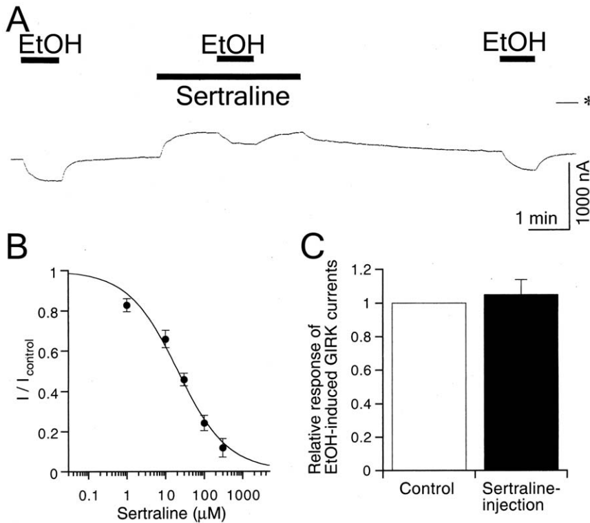
Figure 6. Effect of sertraline on ethanol-induced GIRK currents. (A) Current responses to 100 mM ethanol (EtOH), 100 mM EtOH in the presence of 30 μM sertraline, and 100 mM EtOH in an oocyte injected with GIRK1 and GIRK2 mRNAs. Asterisk indicates the zero current level. Bars show the duration of application. (B) Concentration-dependent inhibition of EtOH-induced GIRK currents by sertraline. I_{\text{control}} is the amplitude of GIRK currents induced by 100 mM EtOH ( 344.2 \pm 40.3 nA, n = 6 ), and I is the current amplitude in the presence of sertraline. (C) Lack of effect of intracellular sertraline on 100 mM EtOH-induced GIRK currents. The amplitude of EtOH-induced GIRK currents after sertraline injection (black bar) was compared with EtOH-induced GIRK currents before the injection (control, white bar) in the same oocyte that expressed GIRK channels ( n = 5 ). Current responses were measured at a membrane potential of -70 mV in an hK solution that contained 96 mM K^+ . All values are expressed as mean \pm SEM. doi:10.1371/journal.pone.0028208.g006
