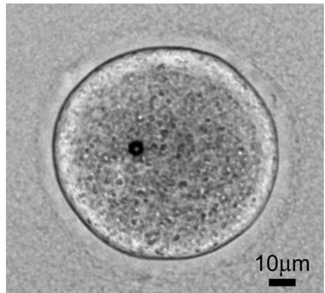
Figure 1. A magnetic bead inside of a mouse oocyte. A photomicrograph of a CD1 mouse oocyte having been injected with a 5 \mu m superparamagnetic bead, and subsequently embedded in fibrin gel, is shown.
