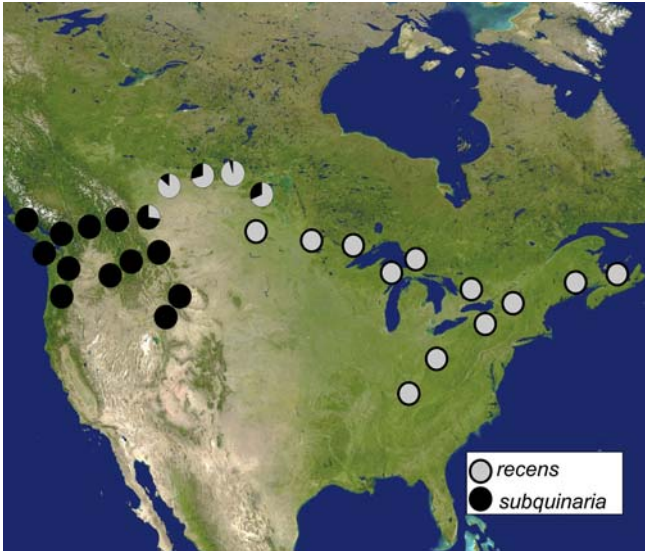
Geographical distributions of Drosophila subquinaria (black) and D. recens (gray), showing allopatric populations of D. subquinaria in the west and D. recens in the east, and sympatric populations in central Canada.
