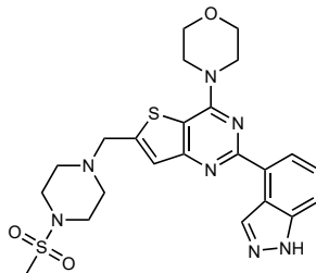
GDC-0941 (pictilisib)
