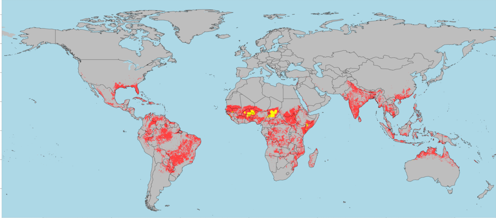
S7 Figure. Regions that fall into different categories with respect to their relationship to peak temperature of 33 °C by 2050 in the month of March. These classifications are based on the RCP 4.5 temperature change scenario [36]. Regions are classified by color according to whether they are projected to remain below (red), newly exceed (yellow), or further surpass (green) the peak temperature of 33 °C for maximizing epidemic growth rate, r . Gray areas are masked from this analysis due to their unsuitability for dengue transmission [39].
