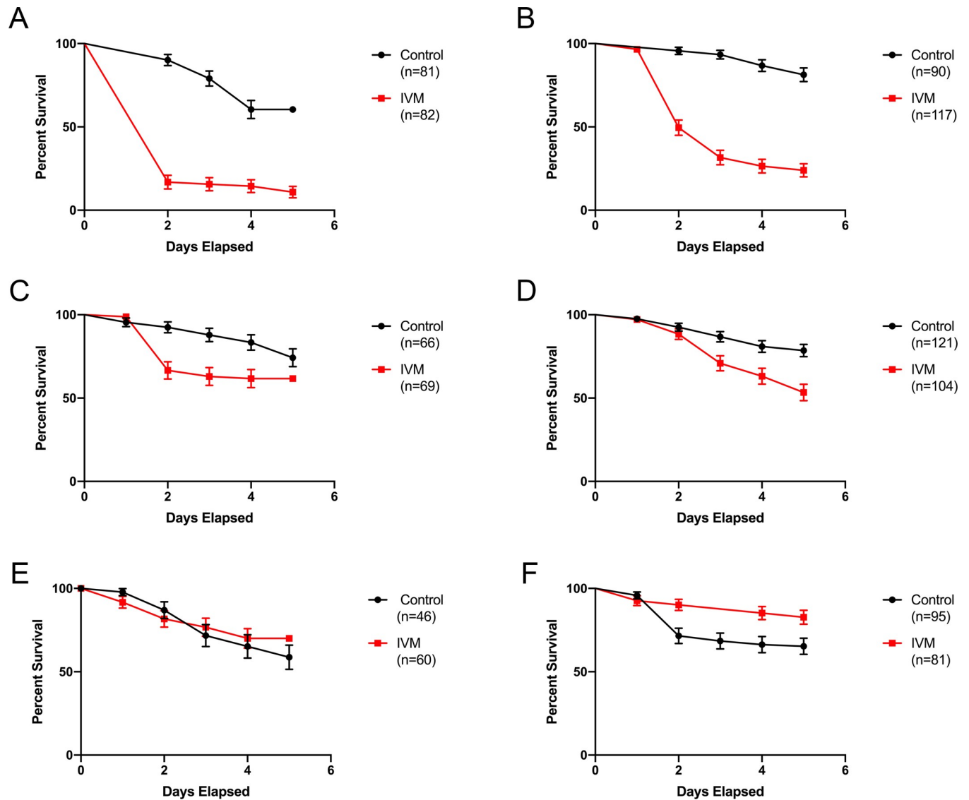
Fig 2. Blood feeding on Ivermec-treated chickens increased Cx. tarsalis mortality. Cx. tarsalis survivorship following direct blood feeding on chickens given Ivermec-formulation diet at a concentration of 200 mg IVM/kg of diet for 3 (left panels: A, C, E) and 7 (right panels: B, D, F) days. (Top panels: A, B) Blood feeding occurred on the last day treated diet was given to the IVM groups. (Middle panels: C, D) Blood feeding occurred one day after treated diet was withdrawn from the IVM groups. (Bottom panels: E, F) Blood feeding occurred on the second day after treated diet was withdrawn from the IVM groups. Error bars indicate standard error.
