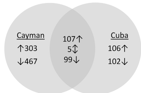
Figure 1. Summary of the genes differentially transcribed between resistant and susceptible strains. The Venn diagram shows the number of genes found significantly ( P < 0.01 ) over- or under-transcribed (>2 fold in either direction) in one or both resistant strains compared to the susceptible New Orleans strain. Upward arrows indicate over-transcribed in resistant strains, downward represent under-transcribed.
