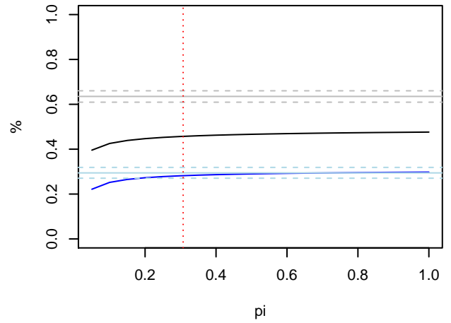
Geometric offspring distribution mean R=1.1
