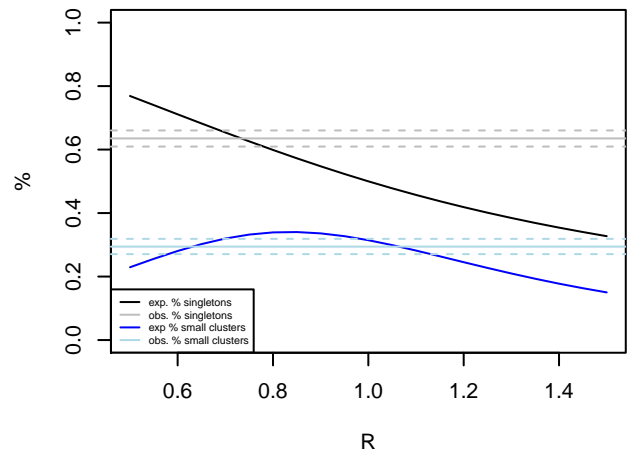
Geometric offspring distribution pi=0.3
