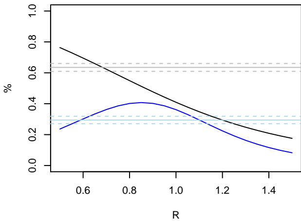
Poisson offspring distribution pi=0.3
