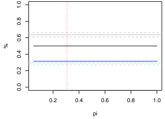
Geometric offspring distribution mean R=1
