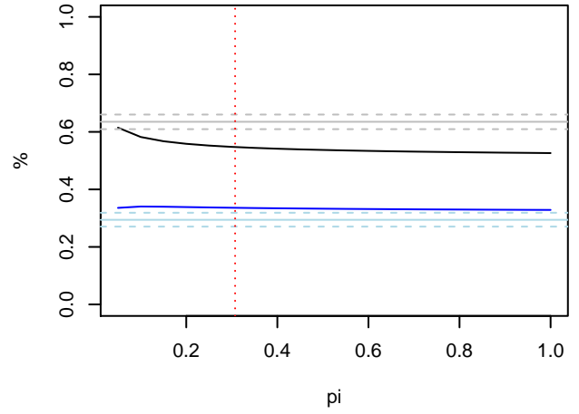
Geometric offspring distribution mean R=0.9
