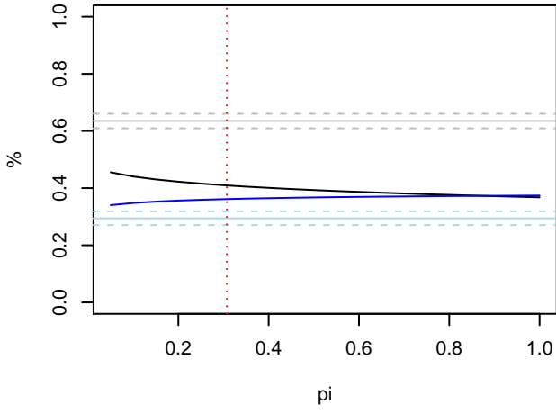
Poisson offspring distribution mean R=1
