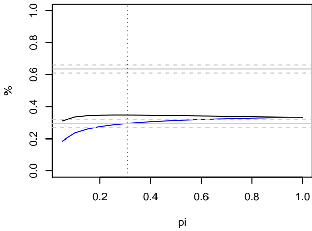
Poisson offspring distribution mean R=1.1
