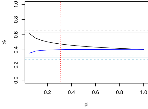
Poisson offspring distribution mean R=0.9
