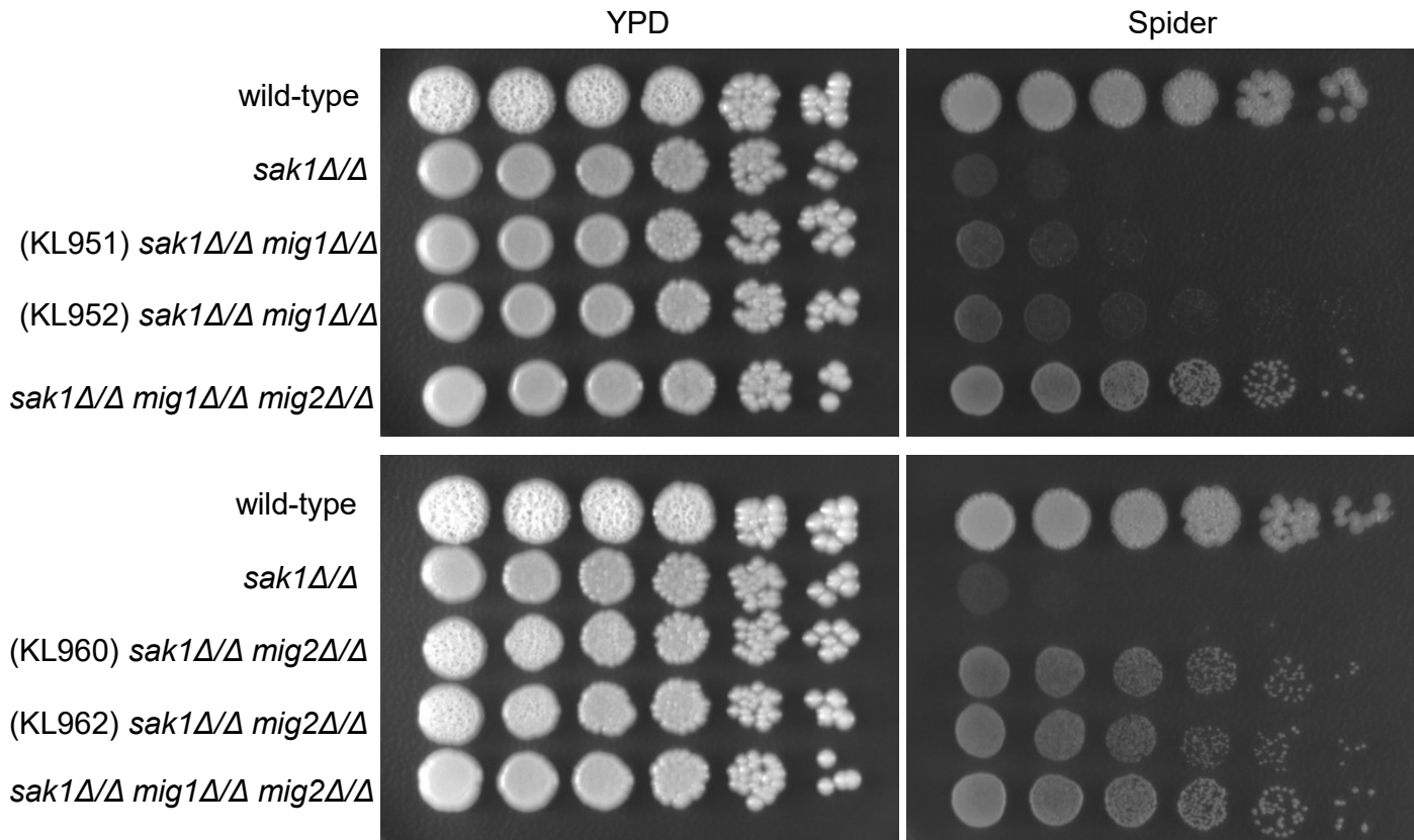
Figure S4. Independent isolates of sak1Δ/Δ mig1Δ/Δ and sak1Δ/Δ mig2Δ/Δ strains show similar growth phenotypes on Spider media.
