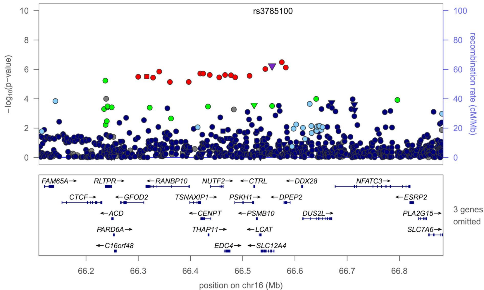
Figure S4C. Association at HDL-C locus LCAT in African Americans. Index SNP rs3785100 ( SLC12A4 -E4G) is the variant showing the strongest evidence of association in trans-ethnic meta-analysis.
