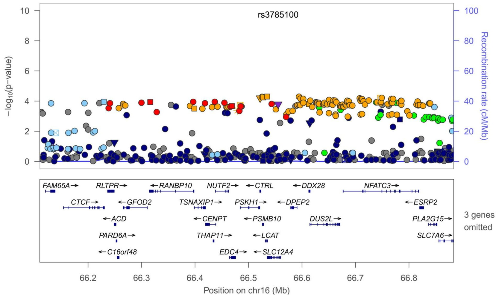
Figure S4A. Association at HDL-C locus LCAT in Europeans. Index SNP rs3785100 ( SLC12A4 -E4G) is the variant showing the strongest evidence of association in trans-ethnic meta-analysis.
