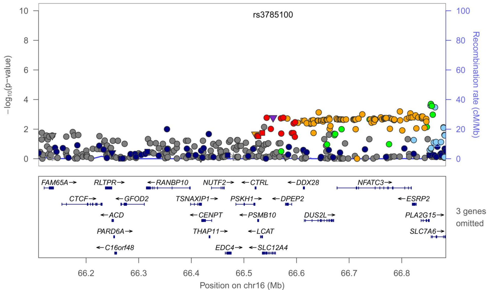
Figure S4B. Association at HDL-C locus LCAT in East Asians. Index SNP rs3785100 ( SLC12A4 -E4G) is the variant showing the strongest evidence of association in trans-ethnic meta-analysis.
