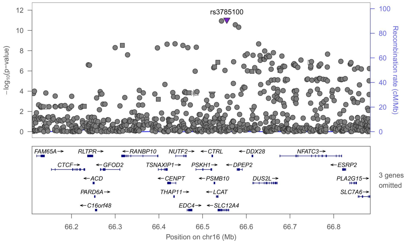
Figure S4D. Association at HDL-C locus LCAT in trans-ethnic meta-analysis.
