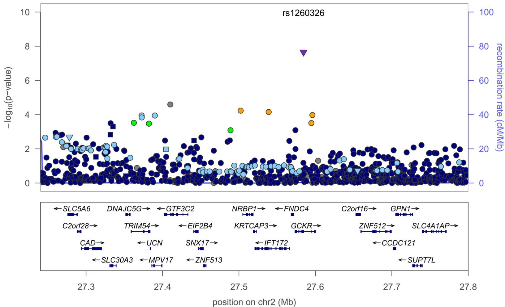
Figure S2C. Association at TG locus GCKR in African Americans. Index SNP rs1260326 (P446L) is the variant showing the strongest evidence of association in trans-ethnic meta-analysis.
