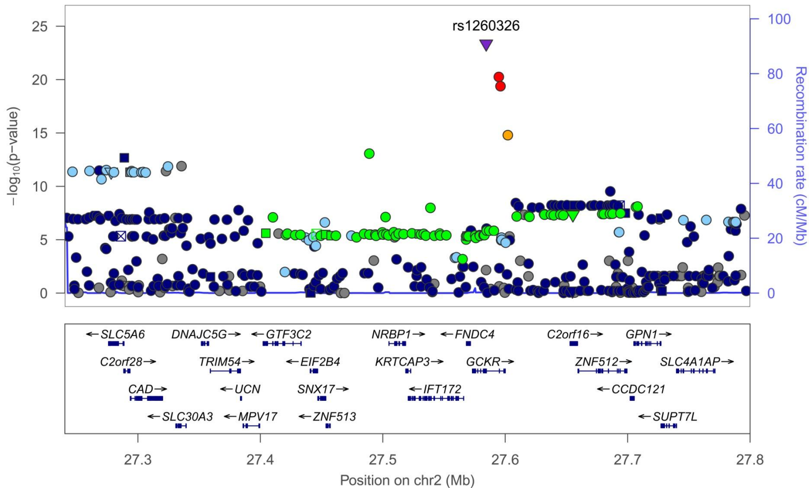
Figure S2A. Association at TG locus GCKR in Europeans. Index SNP rs1260326 (P446L) is the variant showing the strongest evidence of association in trans-ethnic meta-analysis.
