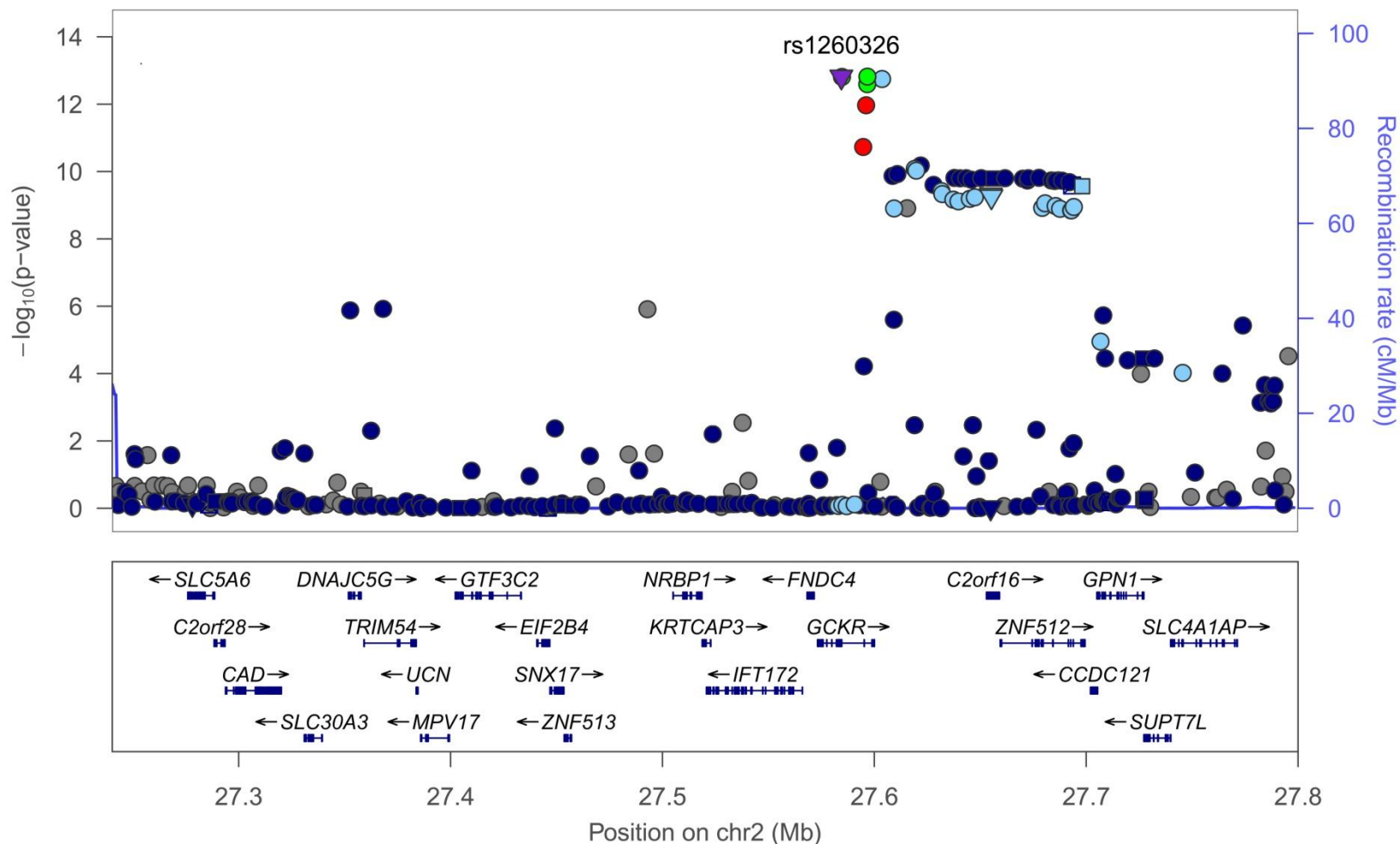
Figure S2B. Association at TG locus GCKR in East Asians. Index SNP rs1260326 (P446L) is the variant showing the strongest evidence of association in trans-ethnic meta-analysis.
