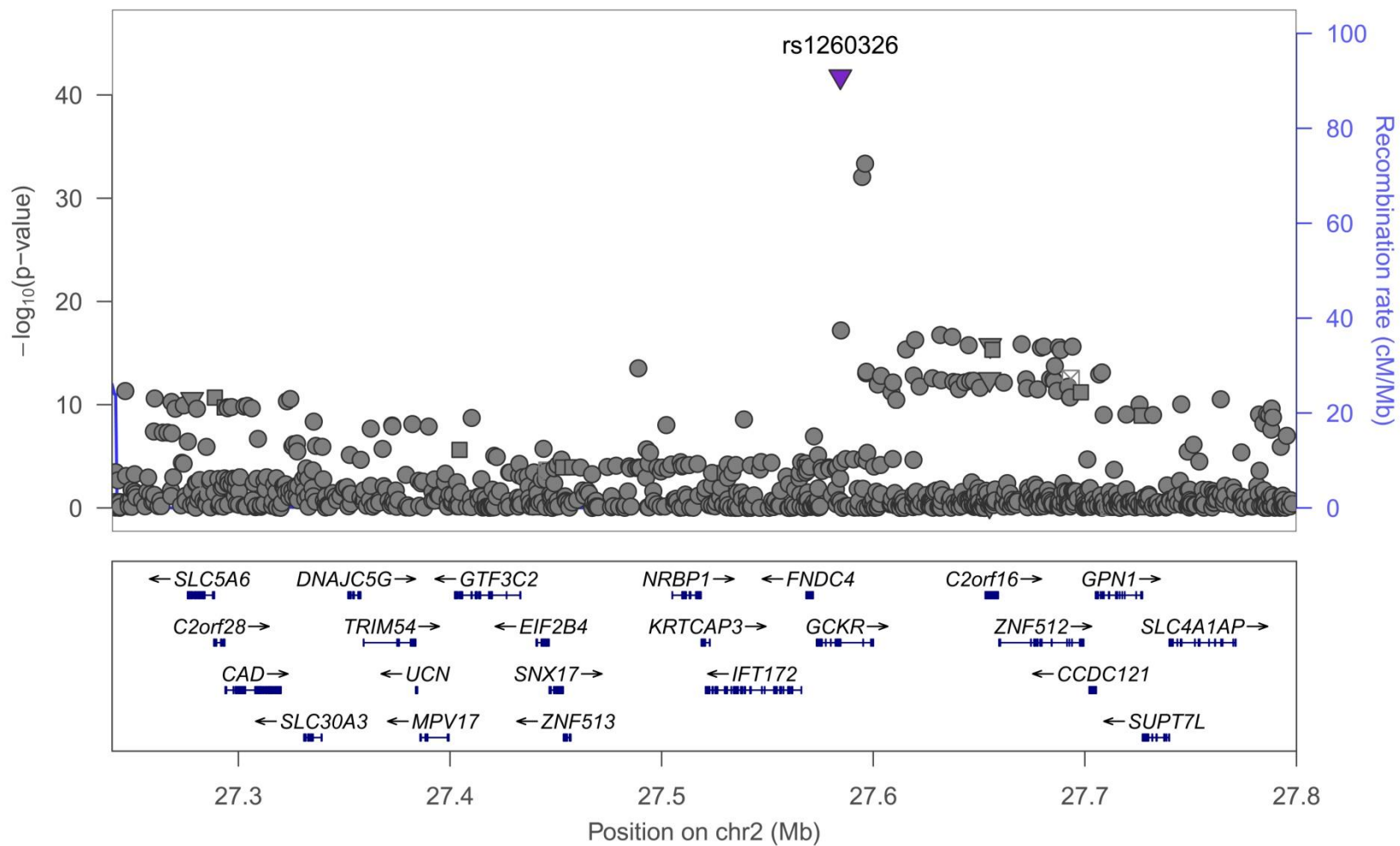
Figure S2D. Association at TG locus GCKR in trans-ethnic meta-analysis.
