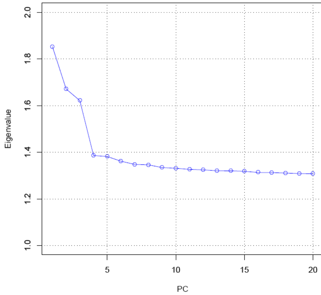
Figure S5. Principal components analysis (PCA) scree plot
