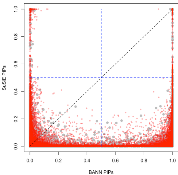
(C) SNP-Level Methods (Polygenic Traits)
