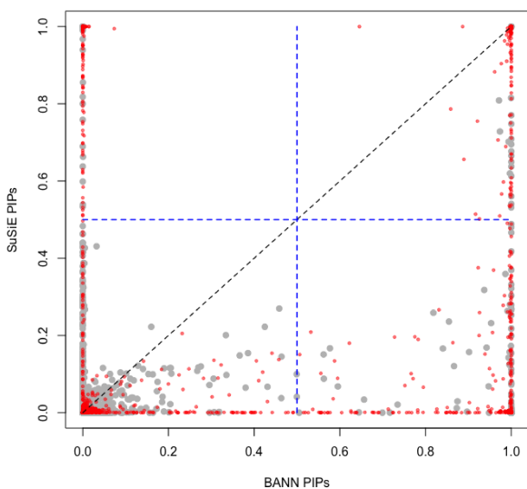
(A) SNP-Level Methods (Sparse Traits)
