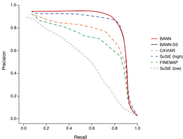
(A) SNP Methods (Sparse Traits)
