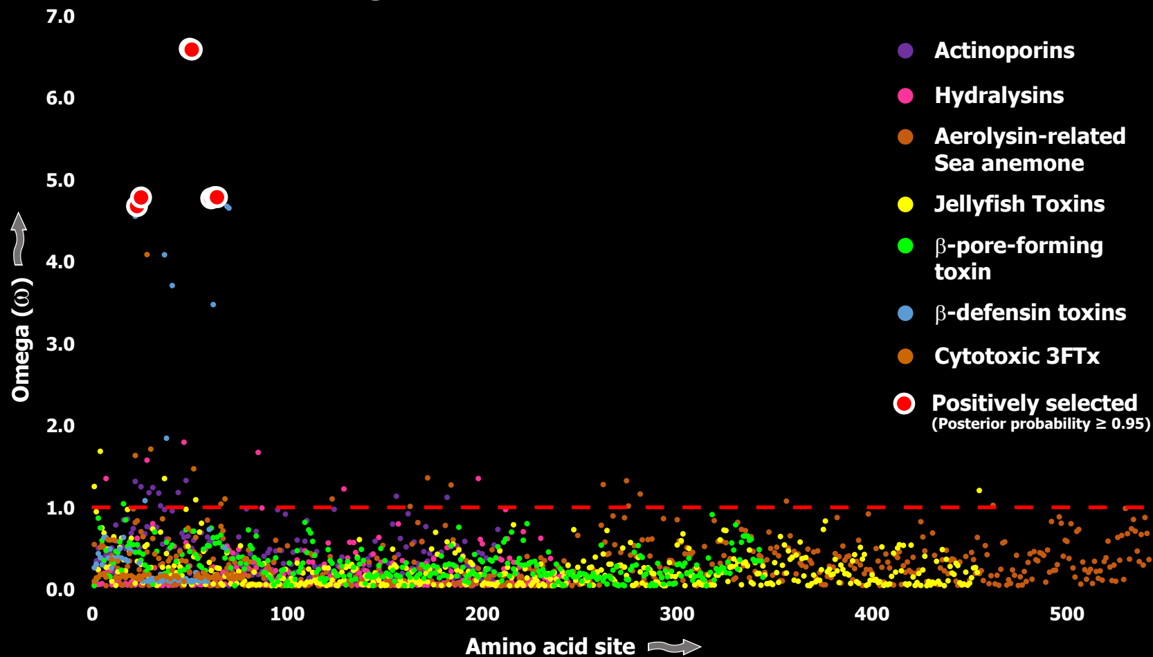
Figure S2: Certain toxins are more constrained than others. A plot of site-specific \omega against amino acid positions for various toxin types is presented. Significantly detected positively selected sites (model 8; Bayes Empirical Bayes approach) are presented as large red circles. The red horizontal line represents the line of neutrality: points above and below this line indicate positive and negative selection, respectively.
