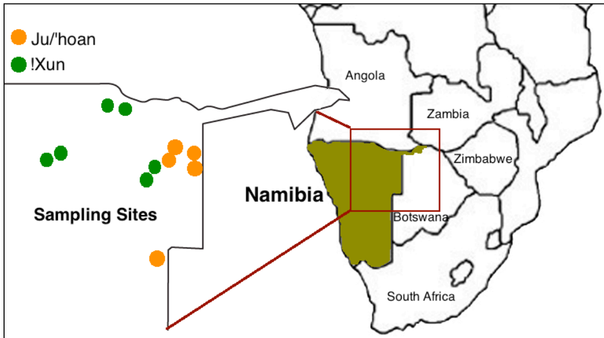
Figure S1. Geographical locations of Khoesan sampling sites included in this study. Study subjects were recruited from 11 locations across the north-western geographical region of Namibia and classified as either Ju/'hoan (orange, n=21) or !Xun (green, n=14). IBD allele sharing resulted in the exclusion of two Ju/'hoan from our study as a result of possible relatedness (total n=19).
