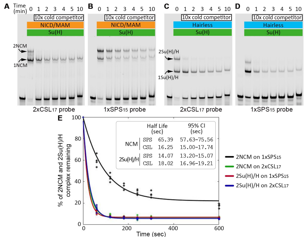
Fig 2. Dimeric NCM complexes dissociate more slowly from the SPS probe than from CSL probe. A–D. EMSAs reveal binding of either the NCM co-activator complex to the 2xCSL_{17} (A) and 1xSPS_{15} (B) probes or the Su(H)/H co-repressor complex to the 2xCSL_{17} (C) and 1xSPS_{15} (D) probes after incubating with 10x unlabeled 2xCSL_{17} competitor probe for the indicated time periods. 3.5nM labeled probe, 80nM Su(H), and 2 \mu M of either Hairless or NICD/Mam was used in the indicated lanes. 35nM unlabeled 2xCSL_{17} probe was used as the cold competitor. E. Percentage of 2xCSL_{17} or 1xSPS_{15} probes bound by 2NCM or 2Su(H)/H complexes over time in the presence of cold competitor probes. Each reaction was repeated four times and the asterisks represent data from each individual experiment. Solid lines represent a fit to decaying exponents (see Materials and Methods). Extrapolated half-lives for each complex and 95% confidence intervals are indicated.
