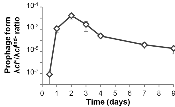
Fig 6. Transient advantage of virulent \lambda cI^* phage. Evolution with time of the proportion of bacteria carrying the virulent \lambda cI^* prophage ( S^- ) on bacteria carrying the \lambda cI^- prophage (L). Means \pm standard error of the mean from 7 mice.
