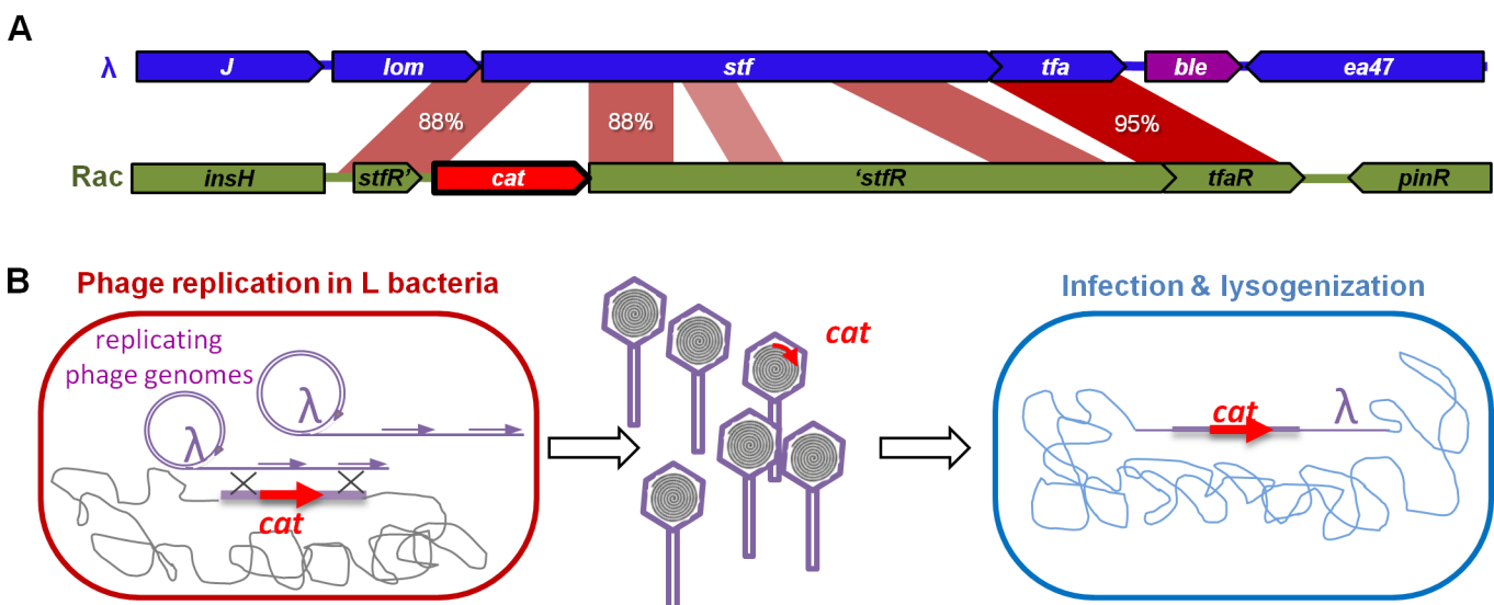
Fig 7. Horizontal gene transfer mediated by \lambda . A) The cat gene conferring chloramphenicol resistance Cm^R (red arrow, cat ) of the lysogenic strain is inserted in the defective prophage Rac. The gene is flanked by regions that share homology with the phage lambda. B) Upon induction, the \lambda phage replicates and can recombine with the bacterial chromosome in such a way that the cat gene is captured by homologous recombination. Bacteria lysogenized by a recombinant phage are resistant to chloramphenicol.
