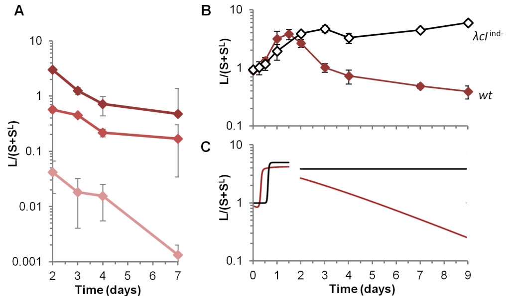
Fig 5. A high in vivo induction rate penalizes lysogens in the absence of susceptible bacteria. A) Evolution of the ratio of lysogen over susceptible lineages ( L/(S+S^L) ) in mice feces after day 2. Means \pm standard deviations from 8, 13 and 4 mice for initial L/S ratios (1:1, 1:10 and 1:100 respectively) are indicated. B) Evolution over 9 days of L/(S+S^L) ratio for wild-type \lambda prophage (brown line) or \lambda cI^{ind-} deficient for induction (black line). Means \pm standard error of the mean from 7 and 12 mice for \lambda cI^{ind-} and wild-type respectively. C) Two-phase temporal simulation of L/(S+S^L) ratio, with a switch at 48h to a \lambda mutant version of the model (i.e. with a = 0 ). The ratio is shown for wild-type phage (red line) or \lambda cI^{ind-} mutant (blue line, with x = 2 \times 10^{-7} ). The initial condition for the first phase is taken from data at time 0, and the initial condition for the second phase (“mutant model”) is taken from experimental data at 48h.
