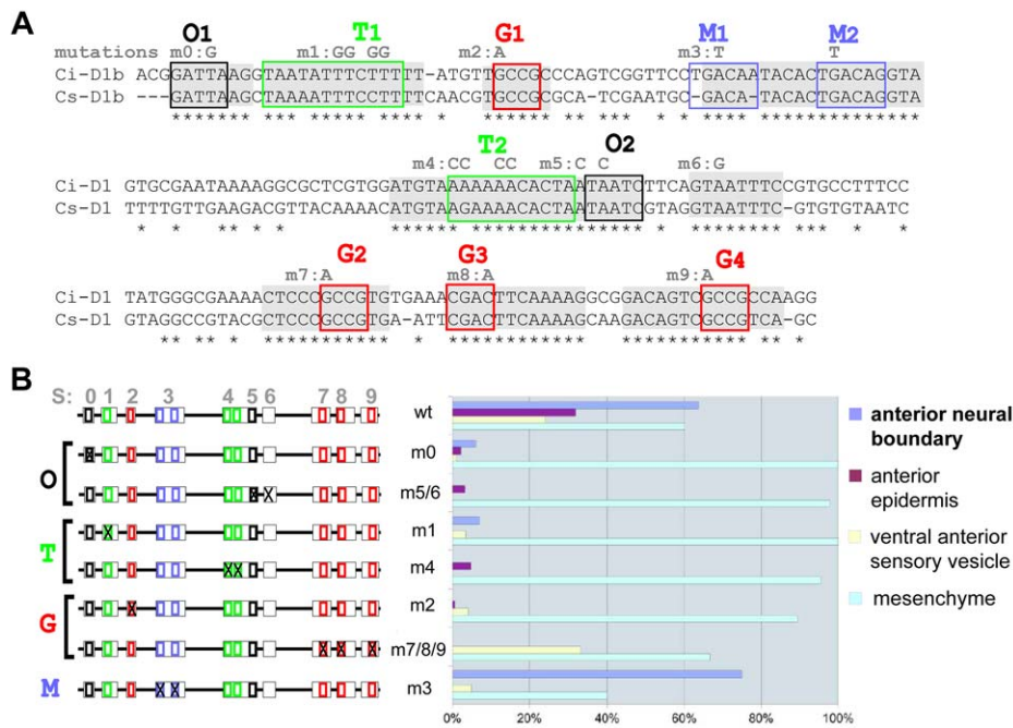
Figure 1. Mutational analysis of D1(bcde) reveals at least three binding sites necessary for its activity. (A) Alignment of D1(bcde) (195pb) between Ci/Cs. Conserved blocks in D1(bcde) with putative transcription factor binding sites (TFBS). Four classes of putative TFBS within ten blocks of conserved sequence: O1 and O2 display the characteristic GATTA/TAATC core sequence that is known to bind K50 Paired -related homeodomain proteins, including otx/otd , pitx and gooseoid . Putative Fox protein binding sites were identified in the blocks called T1 and T2 (T/A-rich). Blocks M1 and M2 show similarity to known binding sites of the TALE-class Meis /TGF1 homeodomain proteins. Finally, putative Smad1/5/8 binding sites were observed in blocks labelled G1, G2, G3 (G/C-rich). Conserved blocks of nucleotides are highlighted in grey. Putative binding sites are represented by colored boxes. Mutations designed to disrupt the binding specificity of each site are indicated in grey above the sequence (m0 to m9). (B) Schematic representation of D1(bcde) and series of mutations introduced into the pD1bcde:CES2 construct. On the right is shown for each construct the rate of mid-tailbud embryos expressing the lacZ reporter in the anterior neural boundary (anb), the anterior epidermis (ae), the ventro-anterior sensory vesicle (vasv) and the mesenchyme (mes) (wt n = 444; m0 n = 198; m1 n = 56; m2 n = 348; m3 n = 40; m4 n = 58; m5/6 n = 182; m7/8/9 n = 29). Most mutations led to a general reduction of the expression level in all of aforementioned domains, while mesenchyme expression remained high. Only construct m3 (block M1 and M2) retained the activity in the anterior neural boundary. doi:10.1371/journal.pgen.1000912.g001
