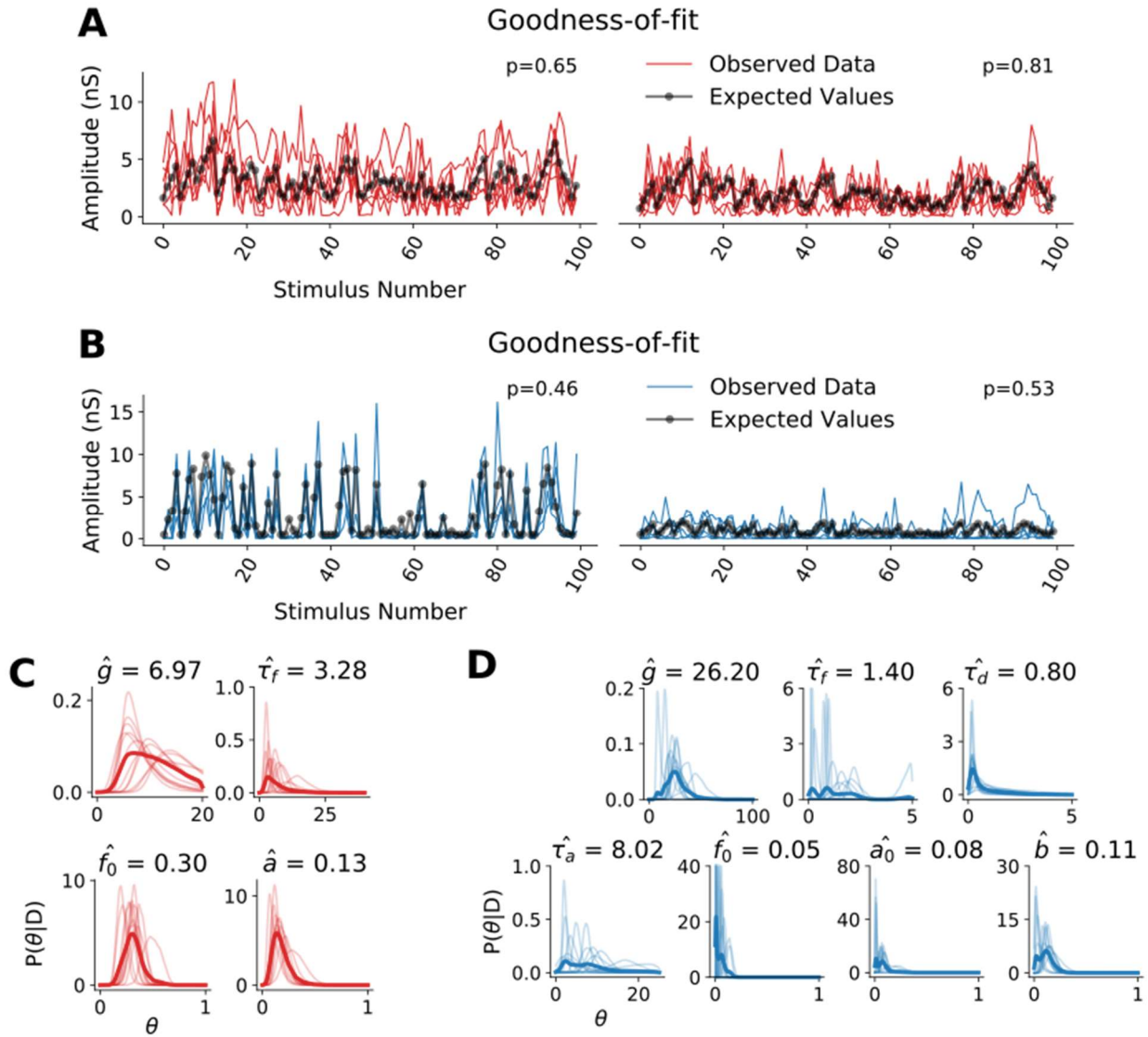
S2 Fig: A-B) Goodness-of-fit for EPSC (A) and IPSC (B) short-term plasticity models assessed by Bayesian posterior predictive p -values. Plots show the observed data for all experiments (EPSCs and IPSCs respectively) together with the expected values from the model before and after the application of 5 \mu M carbachol. p -values close to 0.5 indicate best fit. C-D) Posterior distributions for parameters of best fitting models given data for EPSCs (C) and IPSCs (D).
