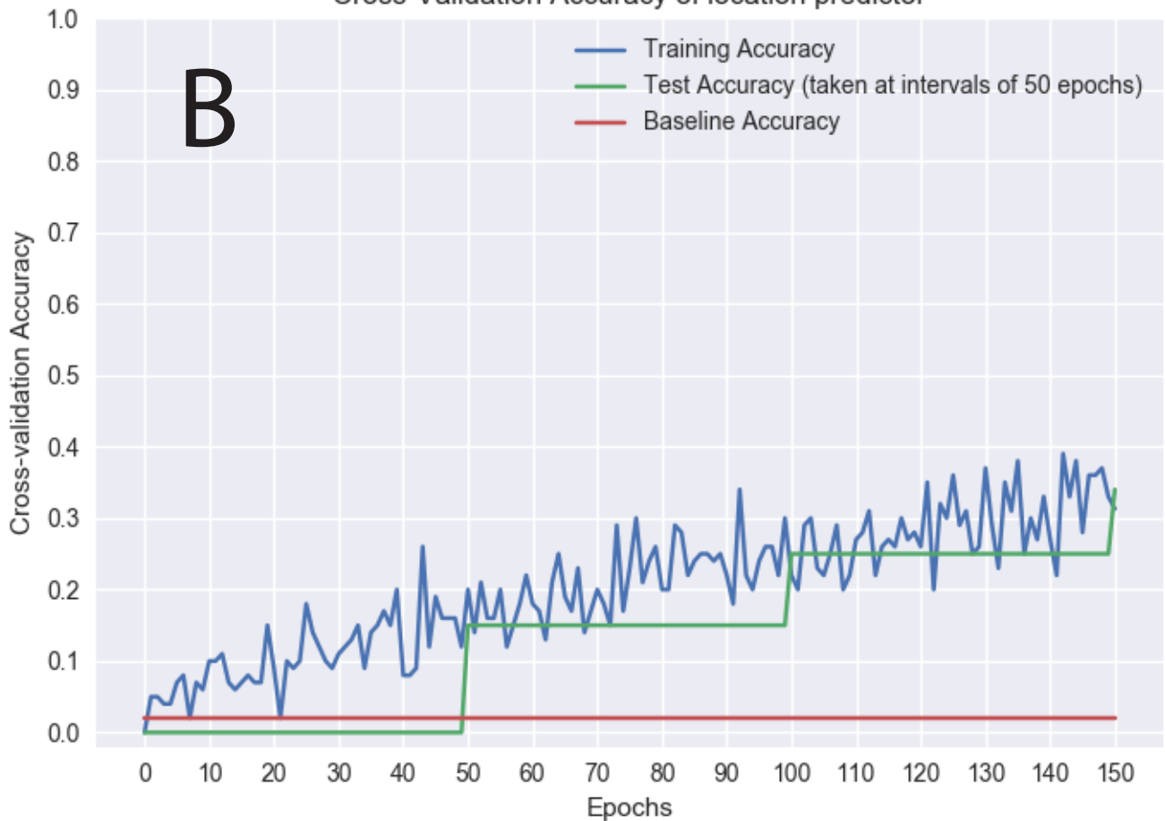
Cross-Validation Accuracy of location predictor
