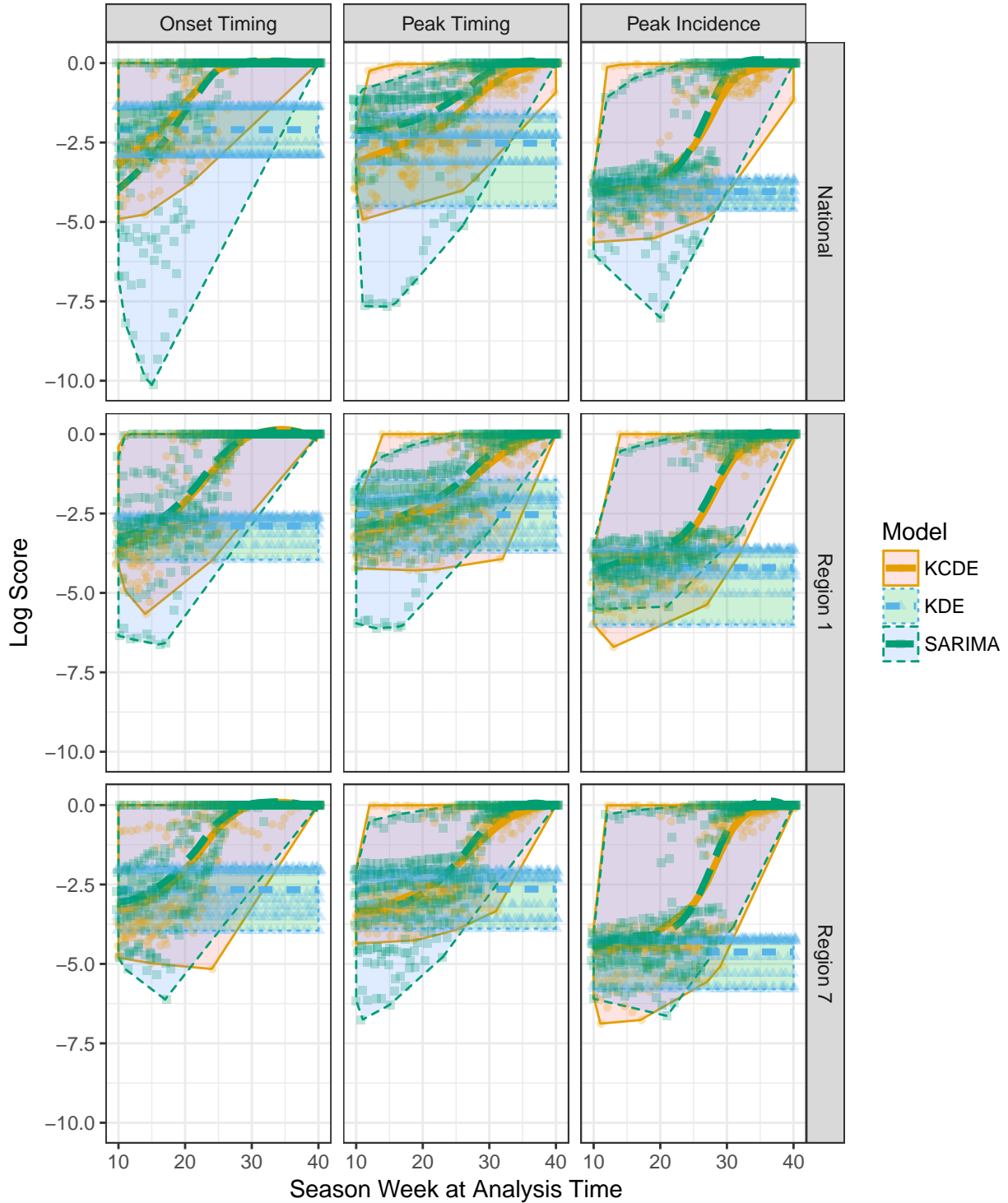
S4 Fig. Log scores achieved by each component model in each week of the season. For each week of the season, log scores are summarized across all seasons in the training phase when all three component models produced predictions. The thick line is a smoothed estimate of mean log score at each week in the season; the shaded region indicates the convex hull of log scores achieved by each model; and the actual log scores achieved in each week are indicated with points.
