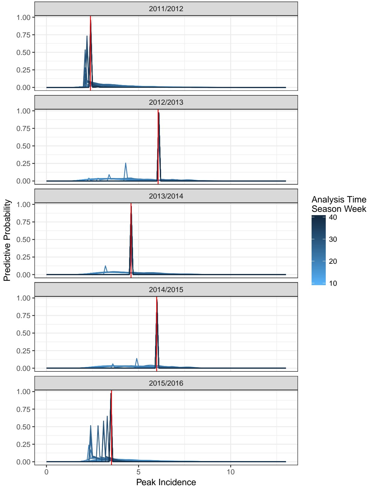
S3 Fig. Predictive distributions for peak incidence. Predictions are shown for just the FW-reg-w method at the national level, faceted by test phase season.
