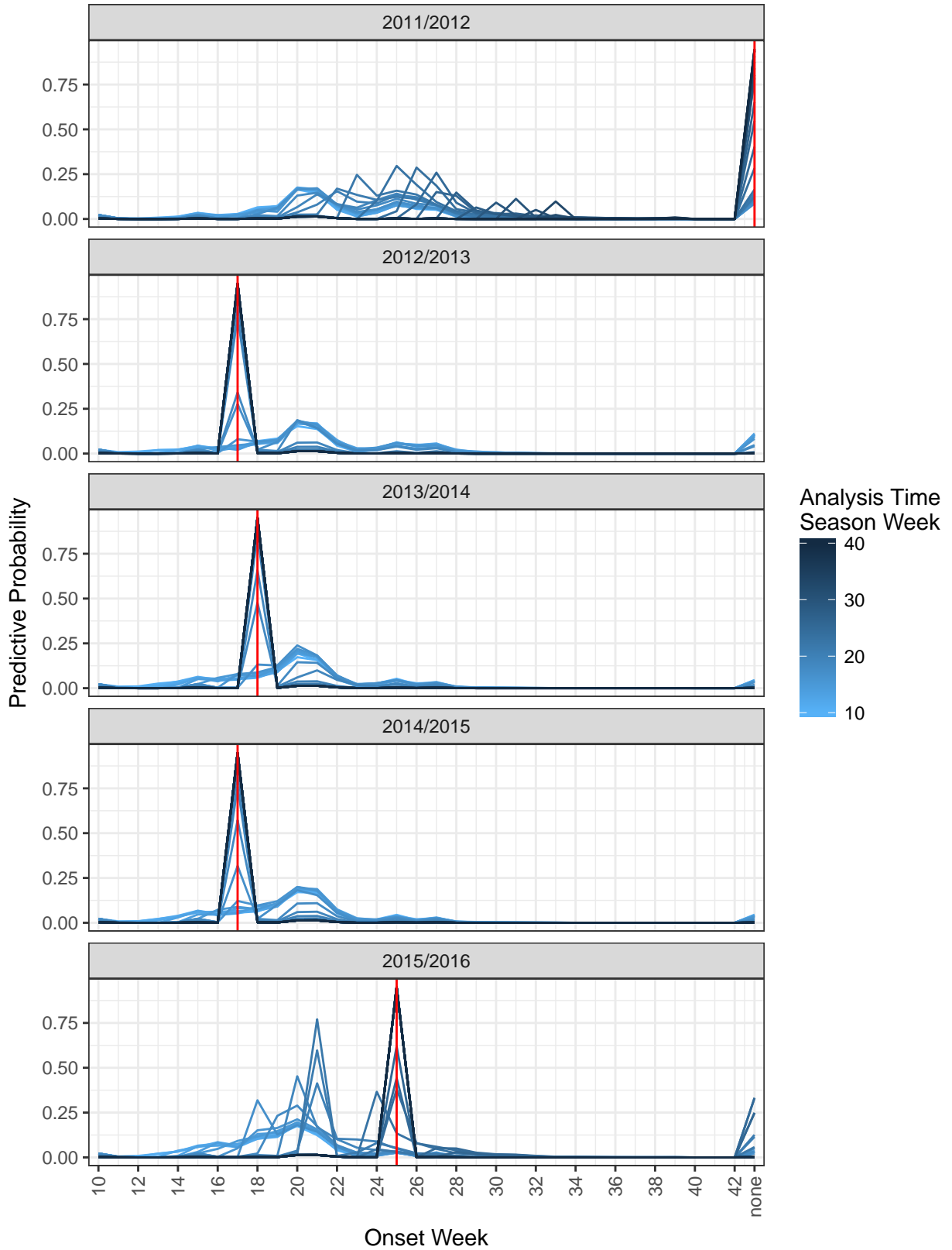
S1 Fig. Predictive distributions for onset timing. Predictions are shown for just the FW-reg-w method at the national level, faceted by test phase season.
