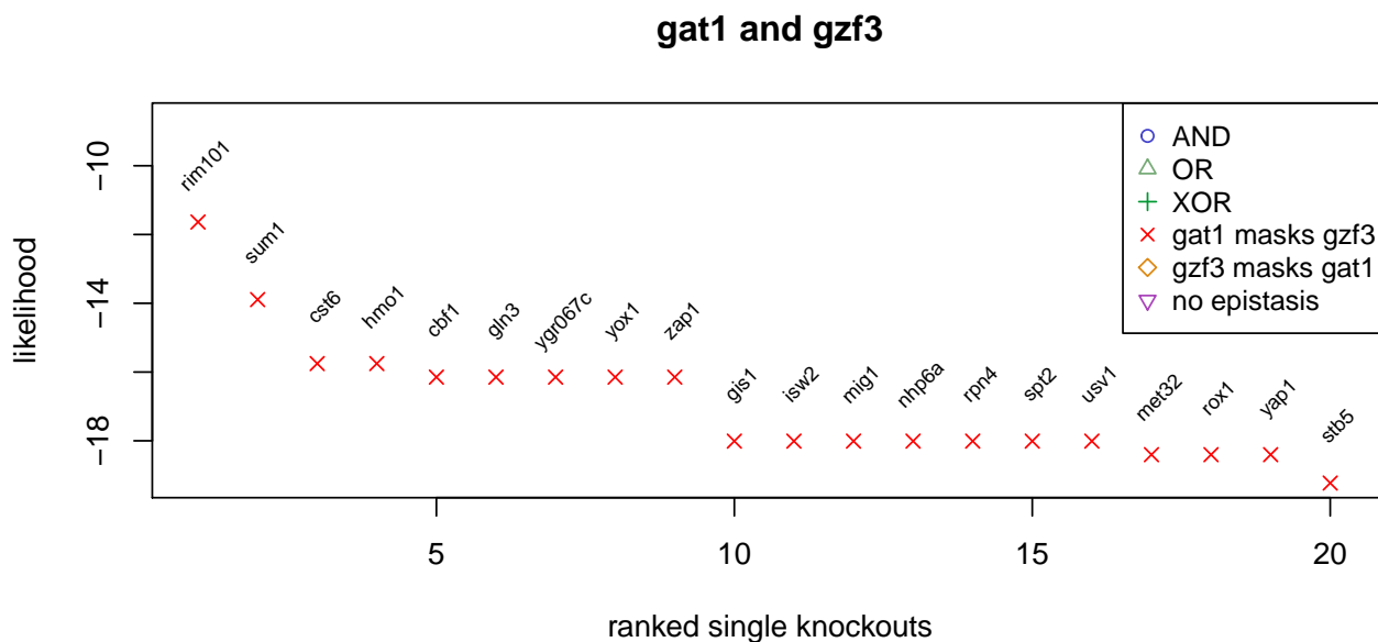
Figure I: Example for one knock-out of the Sameith data set.
