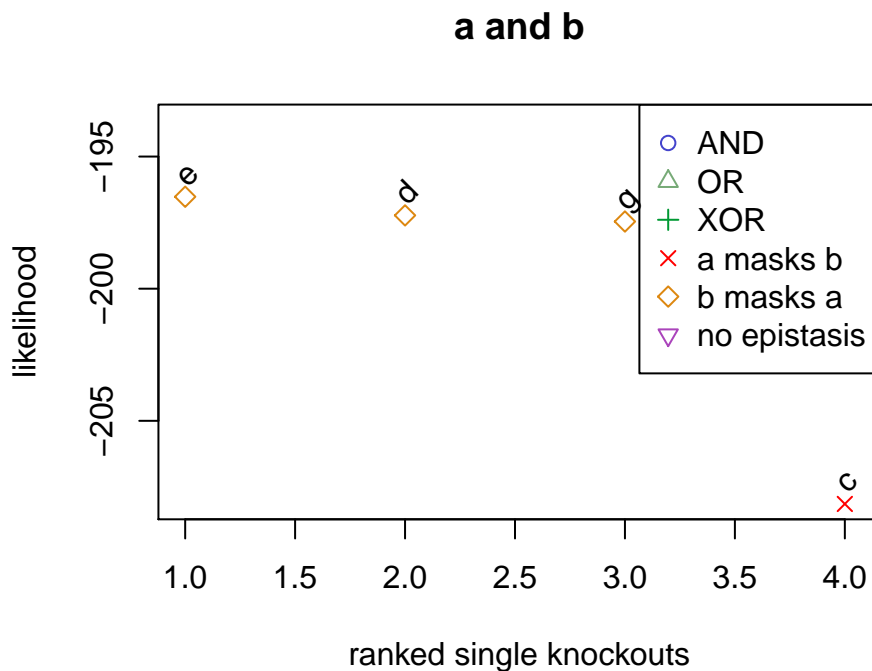
Figure C: Ranked modulators for one double knock-out.
