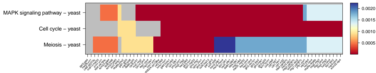
Figure O: Enrichment of Sameith modulators by KEGG pathways. Colors refer to false discovery rates. NAs are colored in grey.
