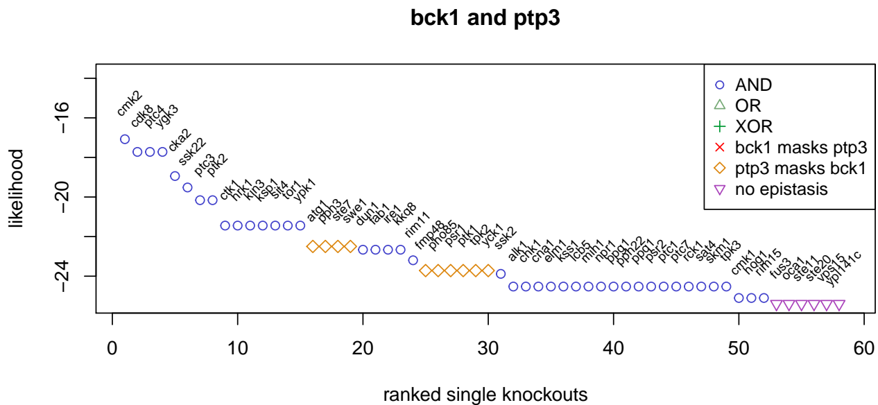
Figure G: Results for one double knock-out of the van Wageningen data set. See ?plot.epiScreen for further parameters.
