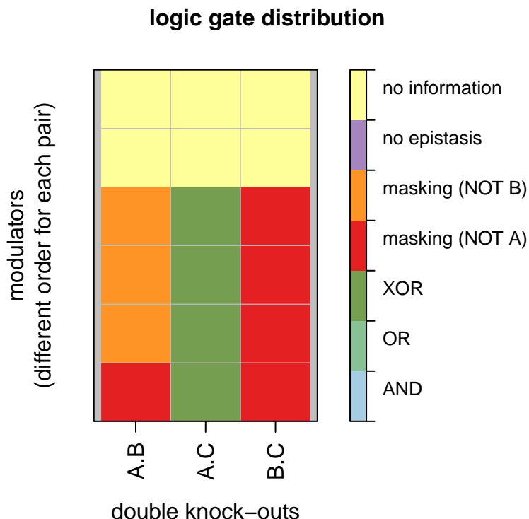
Figure B: Distribution of inferred logics for each double knock-out.
