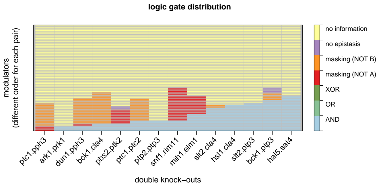
Figure F: Global results for the van Wageningen data set. See the help pages of plot.epiScreen() and HeatmapOP() for additional parameters.
