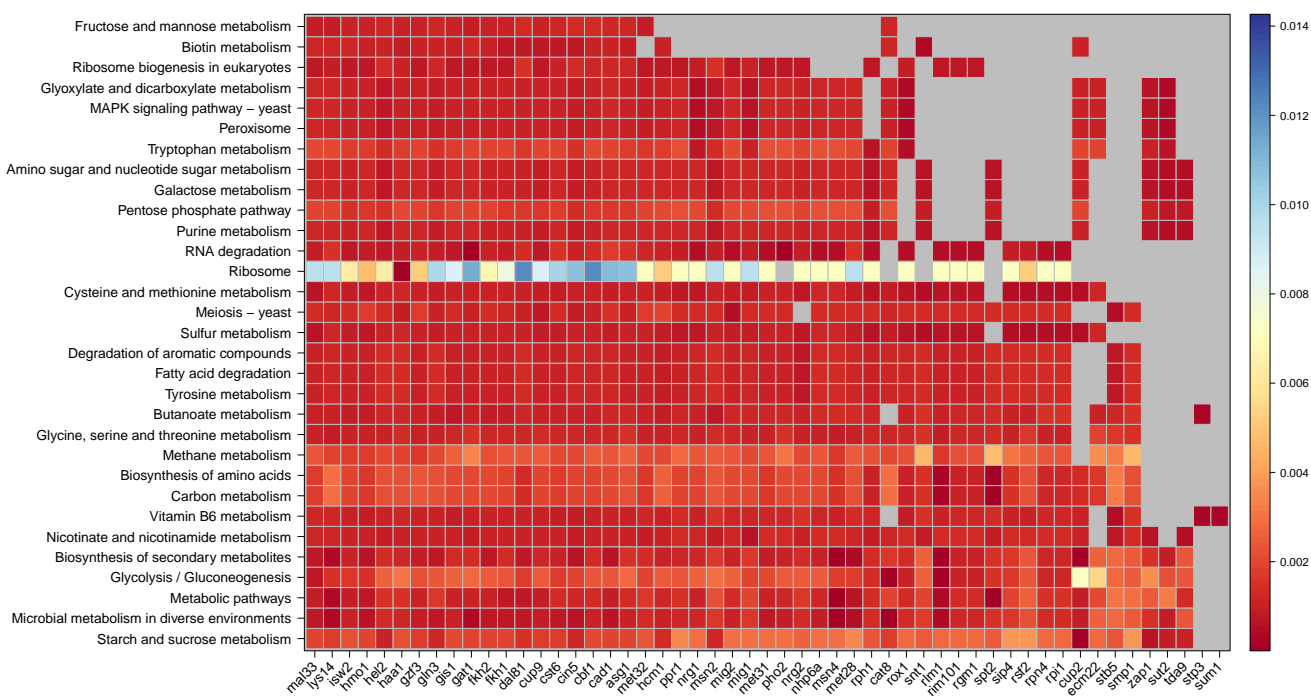
Figure Q: Effect reporter KEGG pathway enrichment (Sameith). Colors refer to false discovery rates. NAs are colored in grey.
