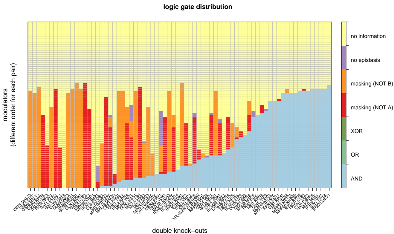
Figure H: Global result for the Sameith data set.
