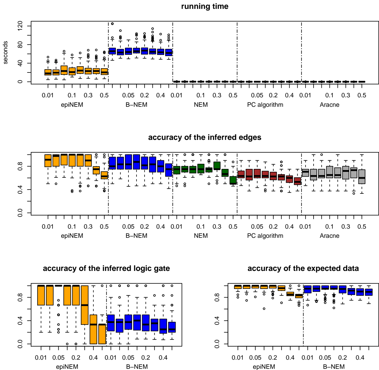
Figure E: Simulation results.
