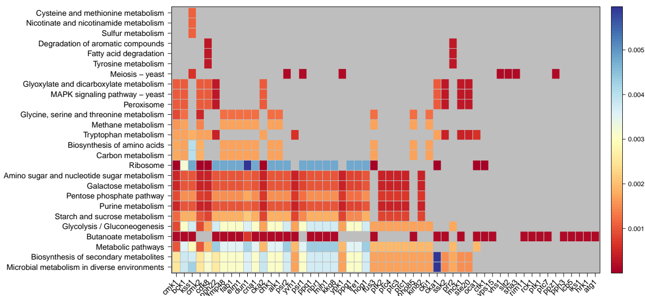
Figure P: Effect reporter KEGG pathway enrichment (van Wageningen). Colors refer to false discovery rates. NAs are colored in grey.
