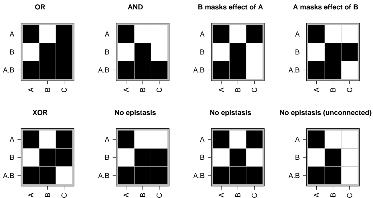
Figure D: Perfect binary effects matrix for each logic.
