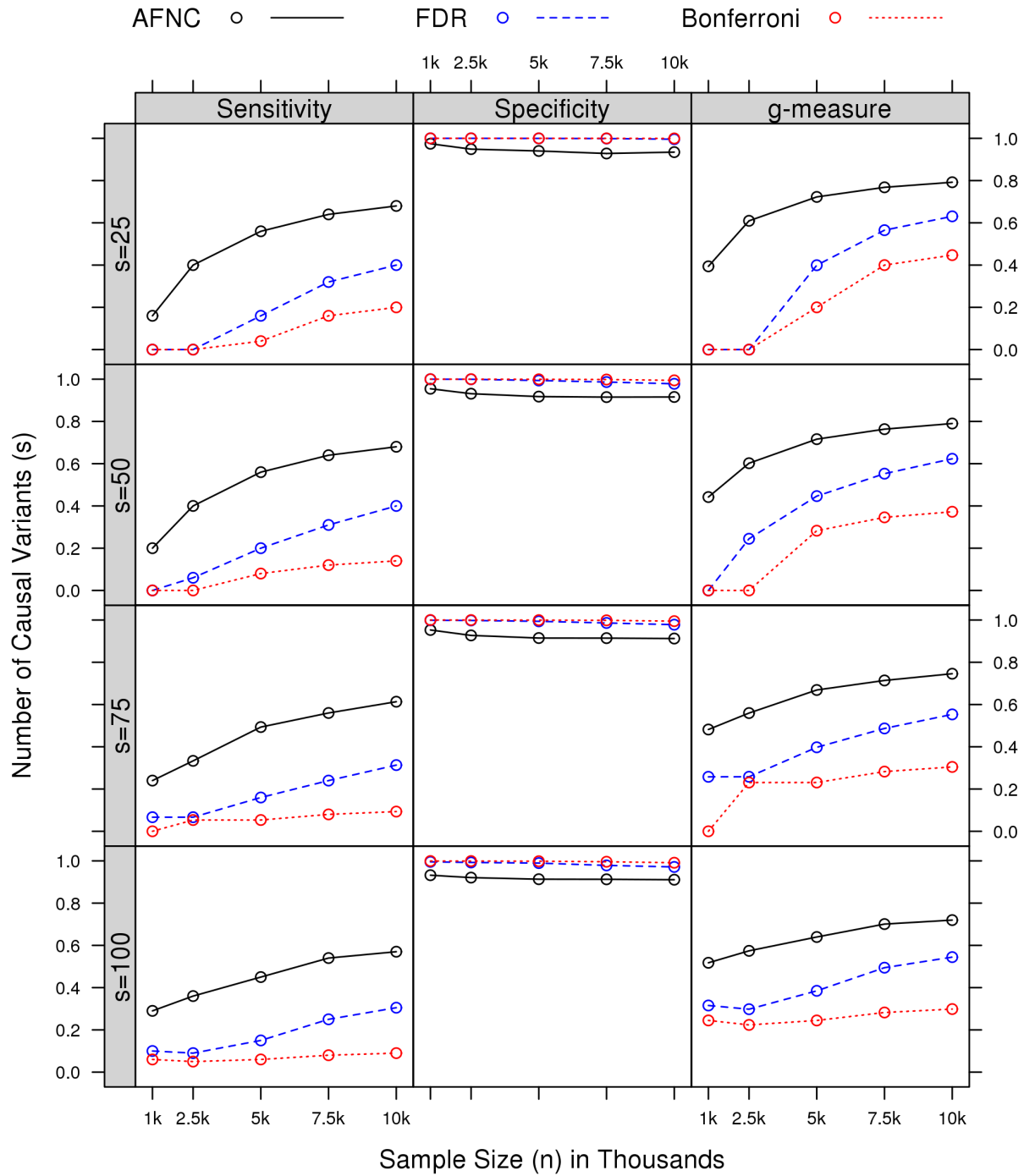
Figure S5: Comparisons across varying sample sizes and numbers of causal variants at C = 0.25 . Performance of AFNC, FDR, and Bonferroni is evaluated in terms of sensitivity, specificity, and g -measure. Results are shown for the effect size multiplier C = 0.25 and d = 100,000 number of variants.
