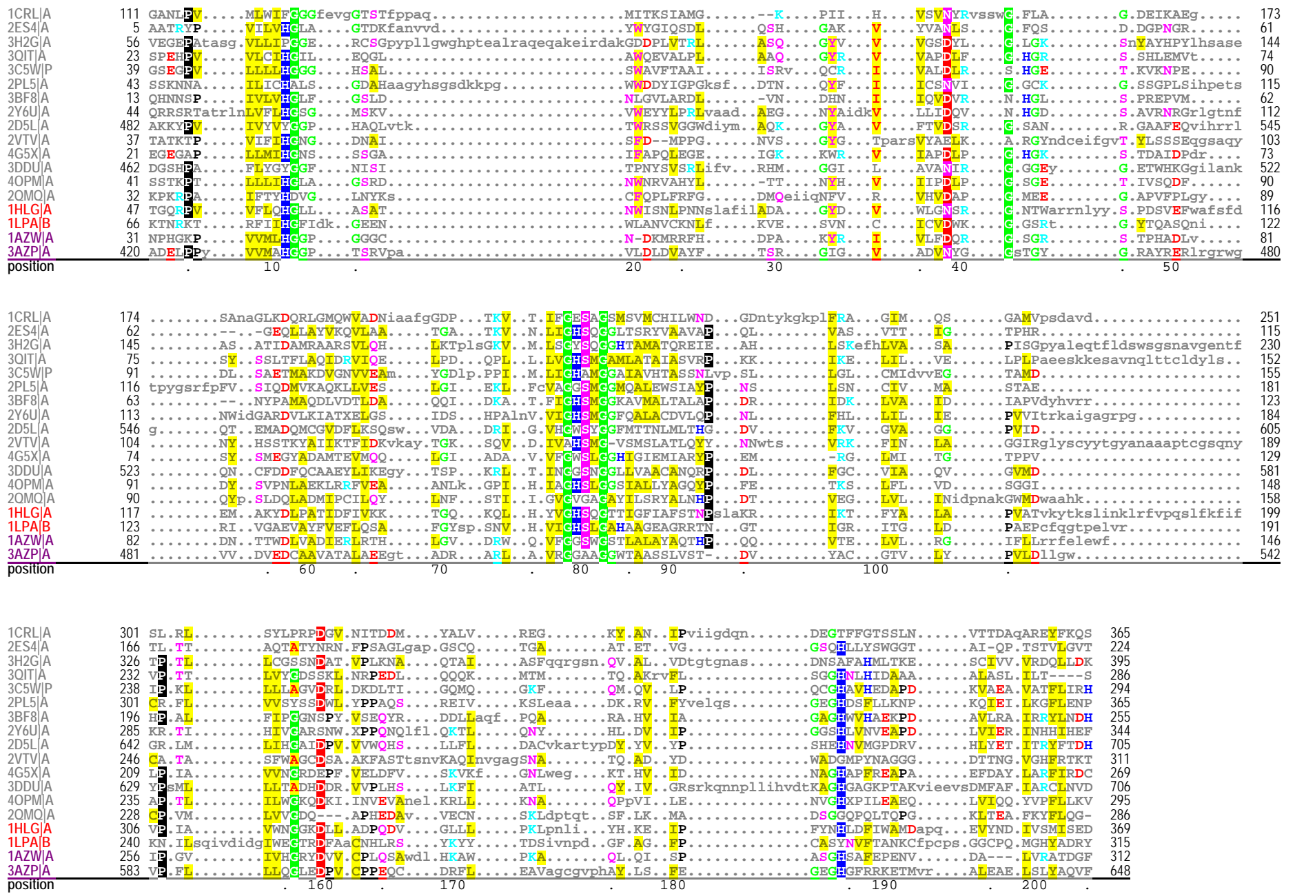
Fig. S4. Representative sequences of known structure from a GISMO alignment of 836 \alpha,\beta -hydrolase fold domains. This corresponds to the same sequences and domain footprint as the MAFFT alignment in Fig. S5.
