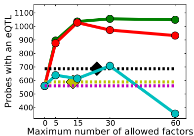
(a) Immediate (cis) eQTLs (t test)
