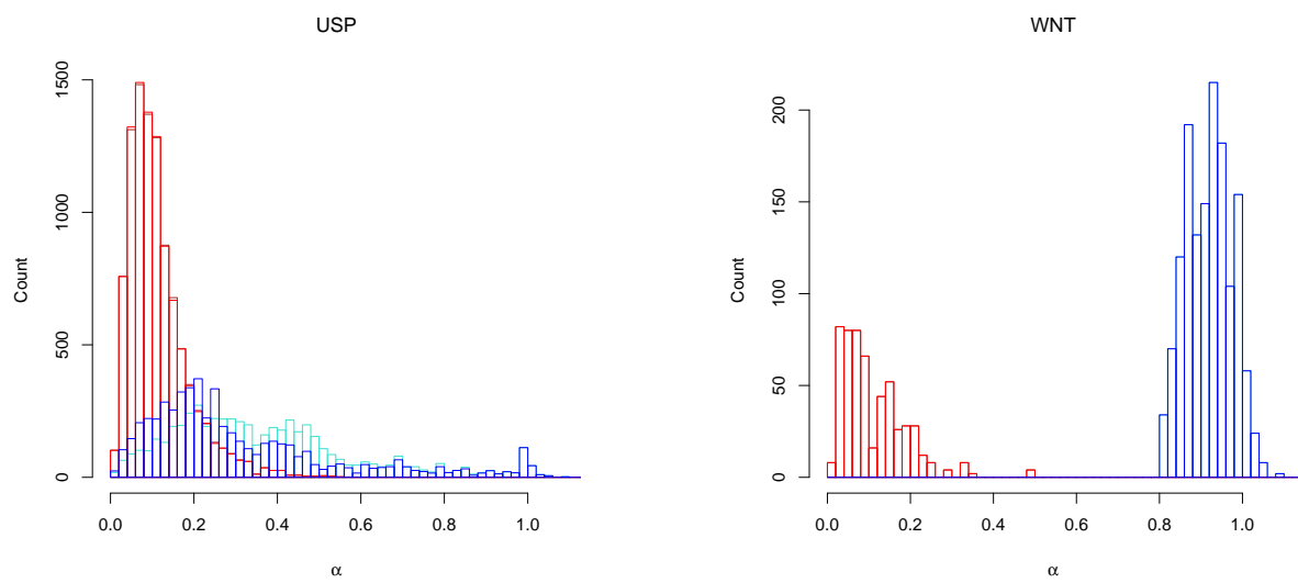
Figure S4: Distributions of alignment coverage calculated with the optimal alignment length only (FF: blue, FO: red) and with combined non-conflicting alignments (FF: turquoise, FO: brown) for all families.
