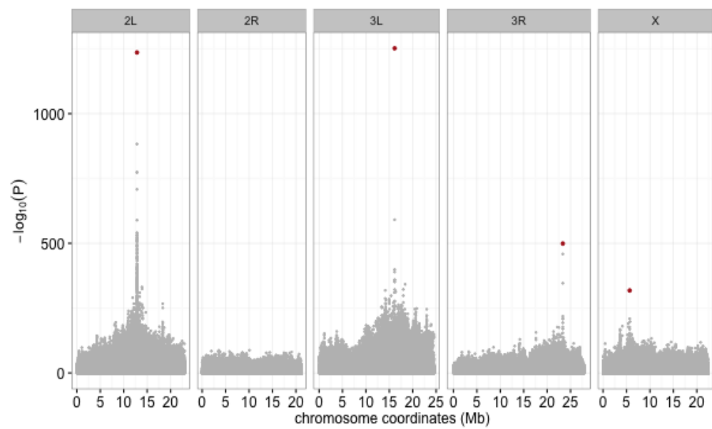
Figure 3: Manhattan plot for a simulated E&R study with 4 QTLs evolving under diminishing returns epistasis.
