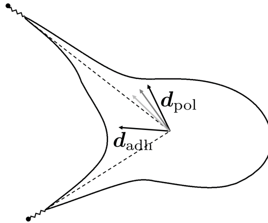
Figure 1: Illustration of polarization of the cell towards the average adhesion direction. The polarization direction d_{pol} rotates with a fixed polarization rate r_{pol} towards the average adhesion direction d_{adh} as seen from the center of mass of the cell. When the polarization direction reaches the average adhesion direction it stops rotating until the average adhesion direction is changed.
