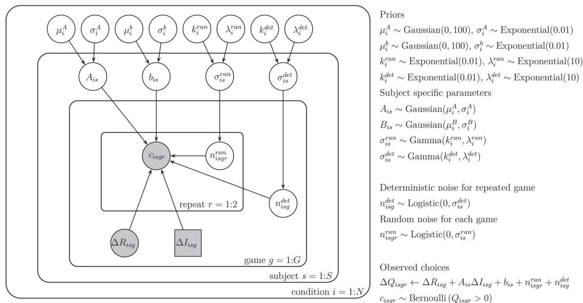
Fig 8. Schematic of the hierarchical Bayesian model using notation of [38].
