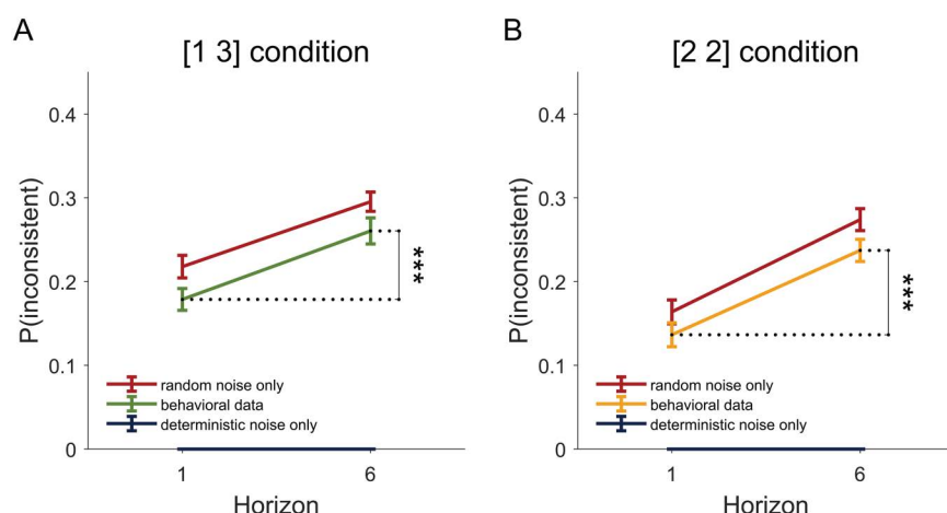
Fig 3. Model-free analysis suggests that both deterministic and random noise contribute to the choice variability in random exploration. For both the [1 3] (A) and [2 2] (B) condition, people show greater choice inconsistency in horizon 6 than horizon 1. However, the extent to which their choices are inconsistent lies between what is predicted by purely deterministic and random noise, suggesting that both noise sources influence the decision.
