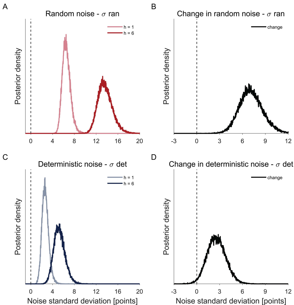
Fig 5. Model based analysis showing the posterior distributions over the group-level mean of the standard deviations of random and deterministic noise. Both random (A, B) and deterministic (C, D) noises are nonzero (A, C) and increase with horizon (B, D).
