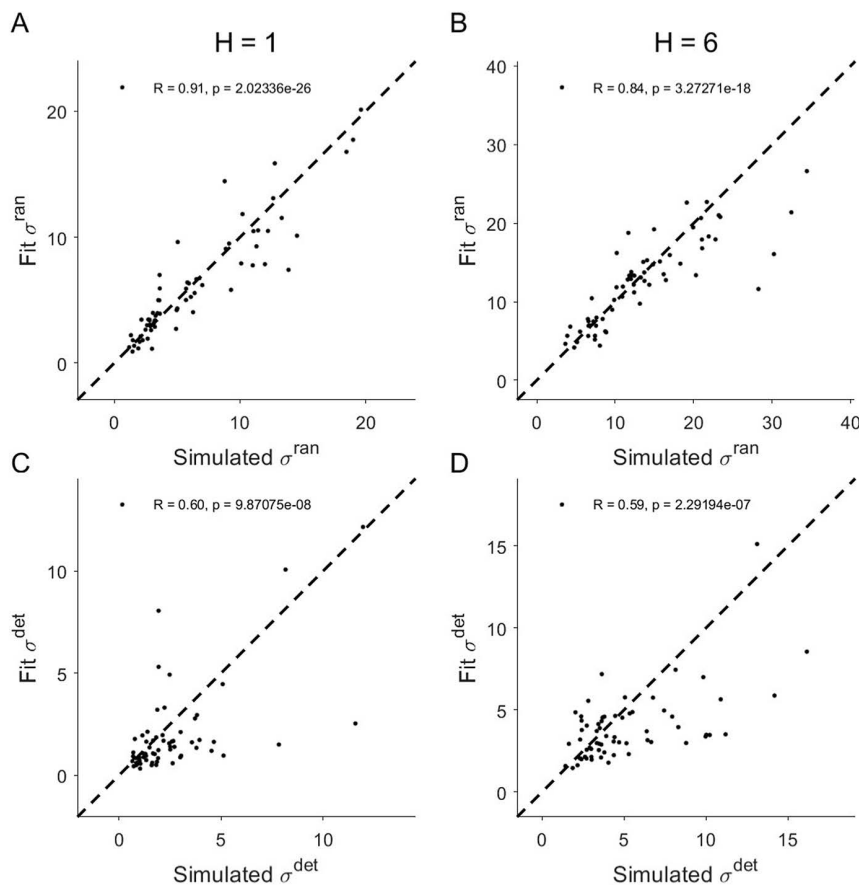
Fig 4. Parameter recovery analysis for random (A,B) and deterministic (C,D) noises in the two horizons.
