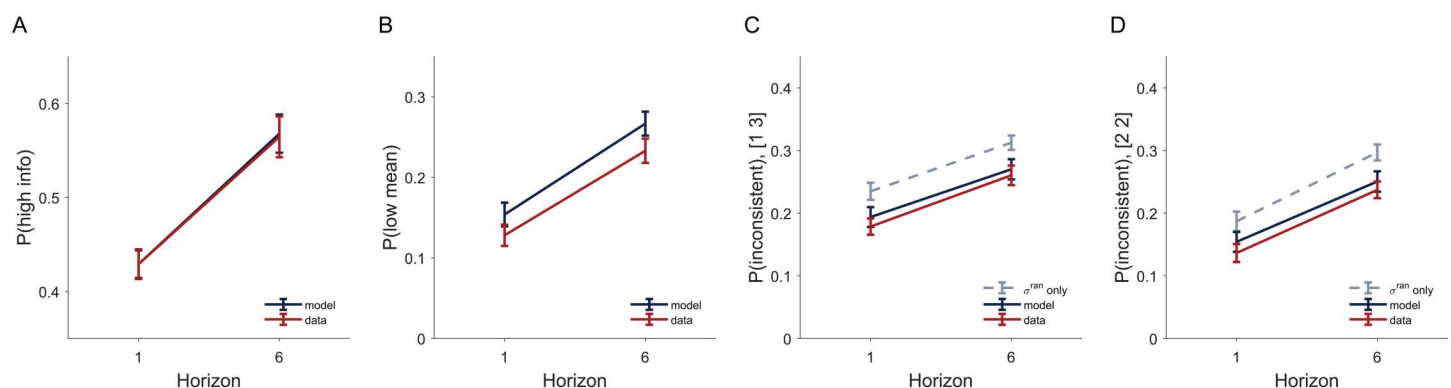
Fig 7. Our model accounts for all qualitative patterns of the data, namely, (A) p(\text{high info}) and (B) p(\text{low mean}) increase as a function of horizon, p(\text{inconsistent}) increases as a function of horizon for both [1 3] (C) and [2 2] (D) conditions and it lies between the pure random and pure deterministic noise prediction.
