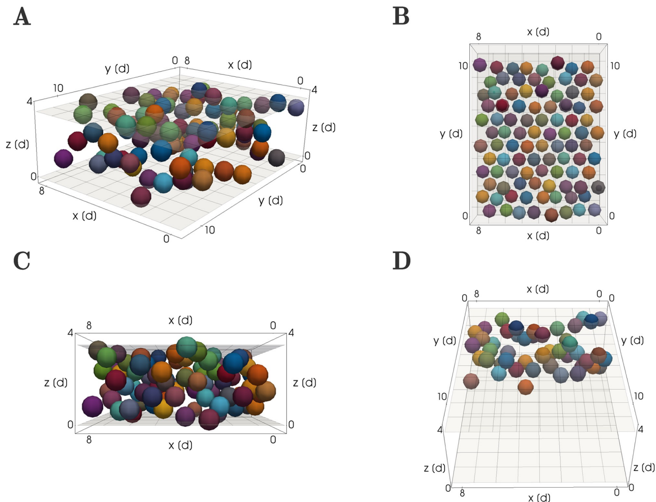
Fig 3. Configuration (i): Cartilage formation from a mesenchymal condensation. Cells were randomly colored and will pass on their color to their progeny. Cells located in close proximity have different colors so that different growing clonal envelopes will be easily distinguishable at later time points in the simulation. (A) General 3D view visualizing the overall shape of the mesenchymal condensation as well as the lower and upper boundary planes situated at their default values of l = 0 and u = 3.5 d . (see Table 1) (B) View of the initial condition from above the cell arrangement in the lateral x - y plane. (C) Sideways view to visualize the spread of the mesenchymal cells in the transversal z direction, showing the positioning of cells between the upper and lower rigid boundary planes. (D) View of the cell population within a subsection of the simulation domain to show cell arrangements within the tissue. Similar visualisations are used to investigate column formation throughout the Results section.
