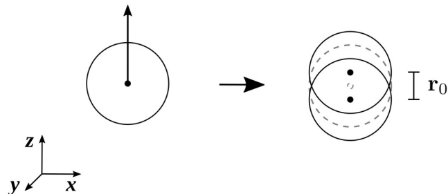
Fig 2. Schematic of cell division implementation used. When a cell is ready to divide, either a random cell division direction is drawn (A), or a cell division direction oriented along the z -axis is used (B). The two daughter cells are placed on a line going through the centroid of the former mother cell, and pointing in the drawn division direction. The cells are placed equidistant from the previous mother cell and separated from each other by the distance r_0 .
