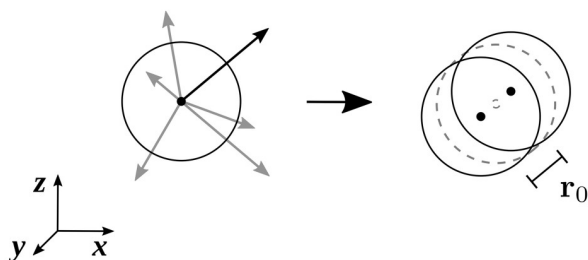
Fig 2. Schematic of cell division implementation used. When a cell is ready to divide, either a random cell division direction is drawn (A), or a cell division direction oriented along the z -axis is used (B). The two daughter cells are placed on a line going through the centroid of the former mother cell, and pointing in the drawn division direction. The cells are placed equidistant from the previous mother cell and separated from each other by the distance r_0 .
