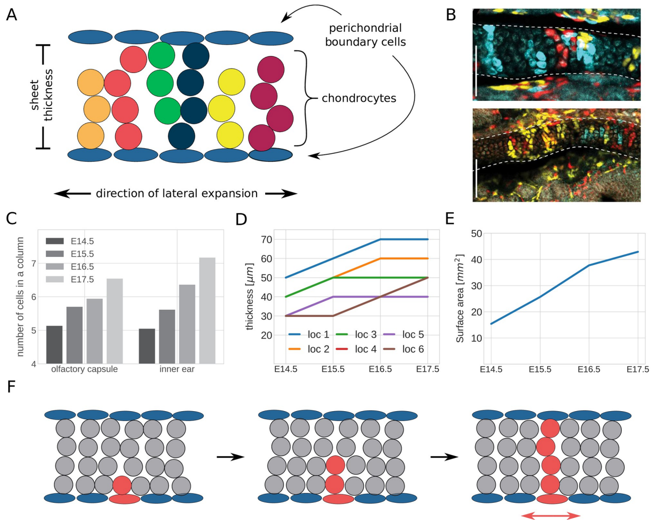
Fig 1. Clonar column growth in sheet-like embryonic cartilage. (A) Schematic of clonar column arrangement; (B) Chondrocyte clones at E17.5 in the olfactory capsule (up) and the inner ear (down) obtained via genetic tracing of neural crest cells at E8.5 using the Plp1-CreERT2/R26Confetti mouse lineage; The scale bars in the lower left corners equal 100 \mu\text{m} . (C–E): Measurements of cartilage geometry in four different developmental stages (E14.5–E17.5) (C) Number of cells per column in the olfactory capsule and inner ear; (D) Cartilage thickness measured at 6 different locations of the nasal capsule; (E) Cartilage surface area of the nasal capsule; (F) Schematic of lateral expansion through clonar column insertion into pre-existing cartilage; Panels (B–F) are adapted from Figs 3, 3S2, 4 and 10 in [1], made available under a Creative Commons CC0 public domain dedication ( https://creativecommons.org/publicdomain/zero/1.0/ ).
