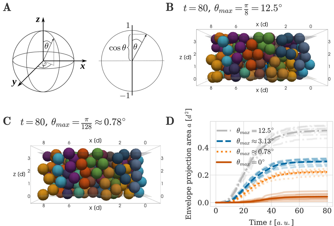
Fig 6. Impact of perturbations in division orientation on column formation. (A) Left: In spherical coordinates a point on the unit sphere is defined by the azimuthal angle \phi and a polar angle \theta . Right: Cosine of the polar angle \theta . Random values of \theta were generated by drawing \cos \theta from a uniform distribution between [\cos \theta_{max}, 1] , ensuring evenly spaced samples on the unit sphere with \theta < \theta_{max} [40]. (B, C) Example simulation snapshots at T = 80 a.u. for two different values of the maximum polar angle \theta_{max} . (D) Envelope projection area over time for different values of the maximum division angle \theta_{max} . The thick line denotes the average over 8 independent repeats of the simulation. The individual data of each simulation are plotted with decreased opacity.
