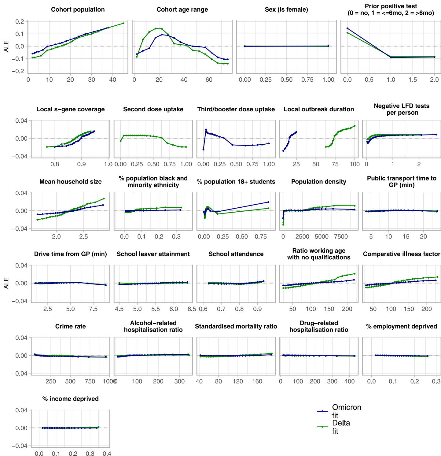
Fig 4. Accumulated local effects across all explanatory variables. For each variable, the x-axis represents the range of values of that variable in the data, and the y-axis (note scale differences for population , age , sex and prior case status ) is the ALE for that variable value. The overall magnitude of the ALE represents the relative size of the effect.
