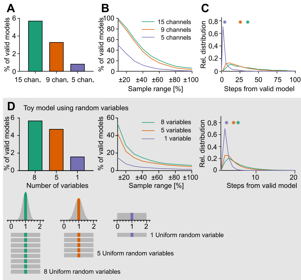
Fig 3. Valid parameter combinations in the fully complex model are more stable as compared to reduced models. A , Percentage of valid random parameter combinations in the total population in the 2-fold range. B , Percentage of valid random parameter combinations in samples with different ranges around the valid reference parameter combination. Each sample contained 5,000 parameter combinations. C , Random walk through the parameter space starting from valid combinations in models of different complexity. Relative percentage distribution of the maximum number of random steps the respective models could undergo without losing their valid GC spiking behaviour. Bin size is 4 steps. Asterisks indicate mean number of steps the corresponding models could undergo while maintaining realistic activity. Performed for 2,000 repetitions per model. A–C , Colours were Green: full model, Orange: 9-channel model, Purple: 5-channel model. D , Reproduction of A–C with a toy model representing the model result as the average value of 1 (blue), 5 (red) and 8 (green) uniform random variables between 0 and 2. Bottom panels , Illustration of how the distribution of solutions becomes narrower when the number of variables is increased. This effect is explained by the law of large numbers while the Gaussian distribution results from the central limit theorem.
