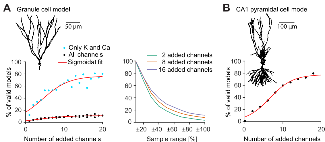
Fig 4. Artificial expansion of ion channel diversity recovers and enhances the proportion of valid parameter combinations in the reduced 5-channel model. A, Populations of expanded dentate GC models with 0–20 added artificial ion channel isoforms. Left panel , The plot shows the percentage of valid parameter combinations in a population of randomly sampled channel densities. Black dots show the populations where all ion channels (including the 8-state Markov chain modelled \text{Na}^+ channel) were sampled in a 0\text{--}2\times range. Blue dots show the populations where only potassium and calcium channels were sampled in a 0\text{--}2\times range. Right panel , Similar plot as in Fig 3B for the black models from the left panel. B, Similar overall analysis as in A but for a CA1 pyramidal cell model [53].
