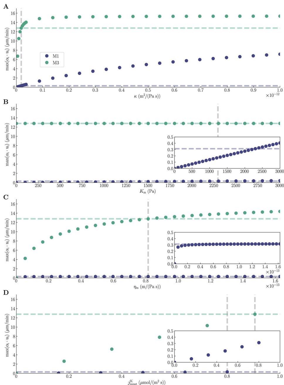
Fig 9. Sensitivity analysis. The maximum superficial fluid velocity, \alpha_i u_i , for different values of the compartmental permeability \kappa (A), membrane stiffness K_m (B), membrane water permeability \eta_m (C), and input flux density j_{\text{input}}^K (D) at t = 200 \text{ s} for modeling scenarios M1 (blue dots) and M3 (green dots). The horizontal dashed lines mark the maximum value of \alpha_i u_i corresponding to the default values of the model parameters, marked with vertical dashed lines. The default value of \kappa was set to be the same in the ICS and ECS, and we changed the two simultaneously by the same amount.
