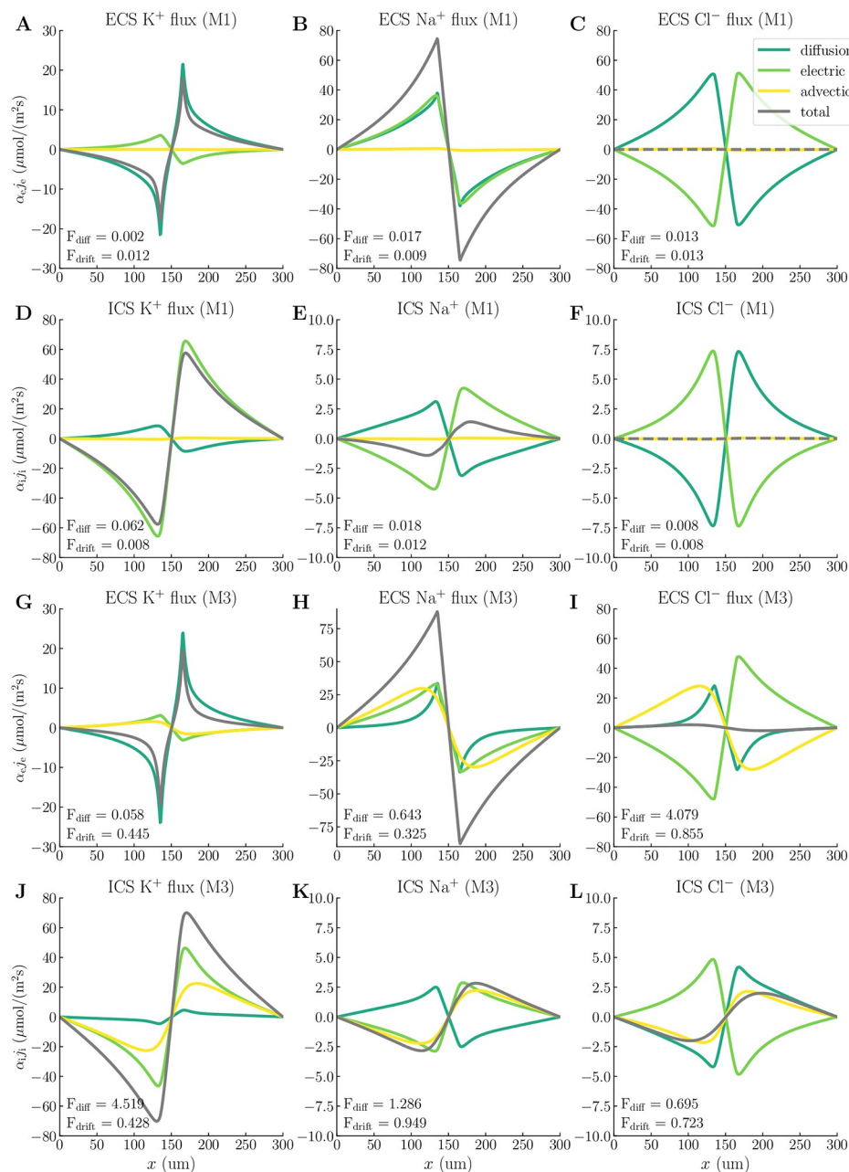
Fig 6. Compartmental ionic fluxes. Spatial profiles of the total compartmental ionic fluxes (grey dashed lines), and their diffusive (dark green lines), electric drift (light green lines), and advective (yellow lines) components at t = 200\text{s} for the different ionic species. Each panel additionally contains the advection/diffusion fraction ( F_{\text{diff}} ) and the advection/electric drift fraction ( F_{\text{drift}} ) for the associated ion species. Panels A-F display fluxes for modeling scenario M1, and panels G-L display fluxes for modeling scenario M3. All fluxes are multiplied by the volume fraction \alpha .
