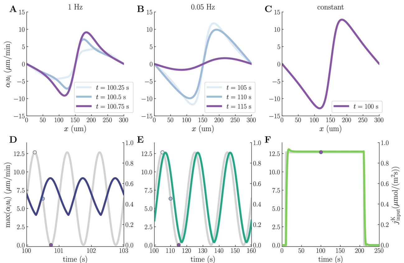
Fig 8. Compartmental fluid velocities during slow, ultraslow, and constant stimuli. The upper panels display spatial profiles of the intracellular superficial fluid velocities at peak (light blue), average (blue), and nadir input (purple) for slow (1 Hz) (A), ultraslow (0.05 Hz) (B), and constant (C) stimuli. The lower panels display the time evolution of the maximum intracellular superficial fluid velocity for the slow (D), ultraslow (E), and constant (F) stimuli, plotted alongside the corresponding \text{K}^+ -input current (gray). The dotted markers in panels D–F correspond to the time points in panels A–C. Note that panels D–F show different time windows on the x-axes. All simulations were run for 250 s and correspond to model scenario M3.
