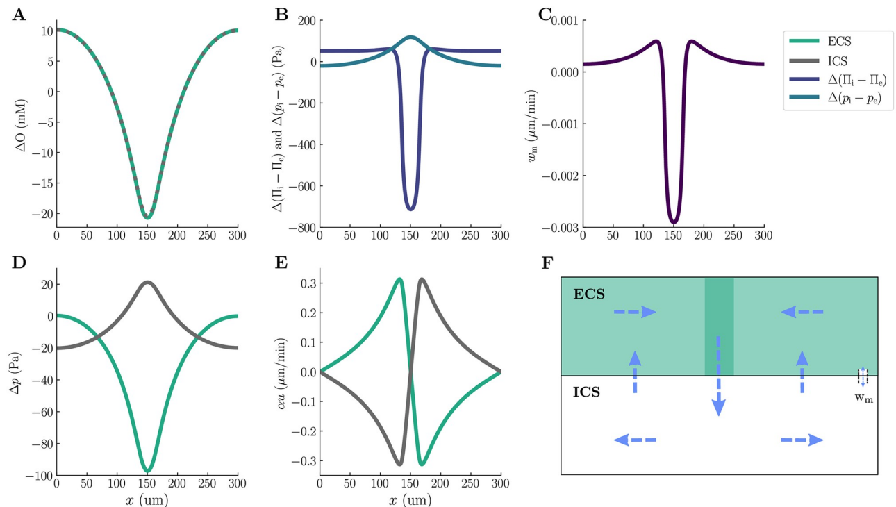
Fig 3. Interplay between transmembrane- and compartmental pressures and fluid velocities (M1). The panels display a snapshot (at t = 200 s) of the spatial distribution of the changes in intra- and extracellular osmolarities (A), osmotic and hydrostatic pressure gradients across the glial membrane (B), transmembrane fluid velocity (C), changes in the intra- and extracellular hydrostatic pressures (D), intra- and extracellular superficial fluid velocities (E), and illustration of the flow pattern (F). All changes are calculated from baseline values, which are listed in Methods.
