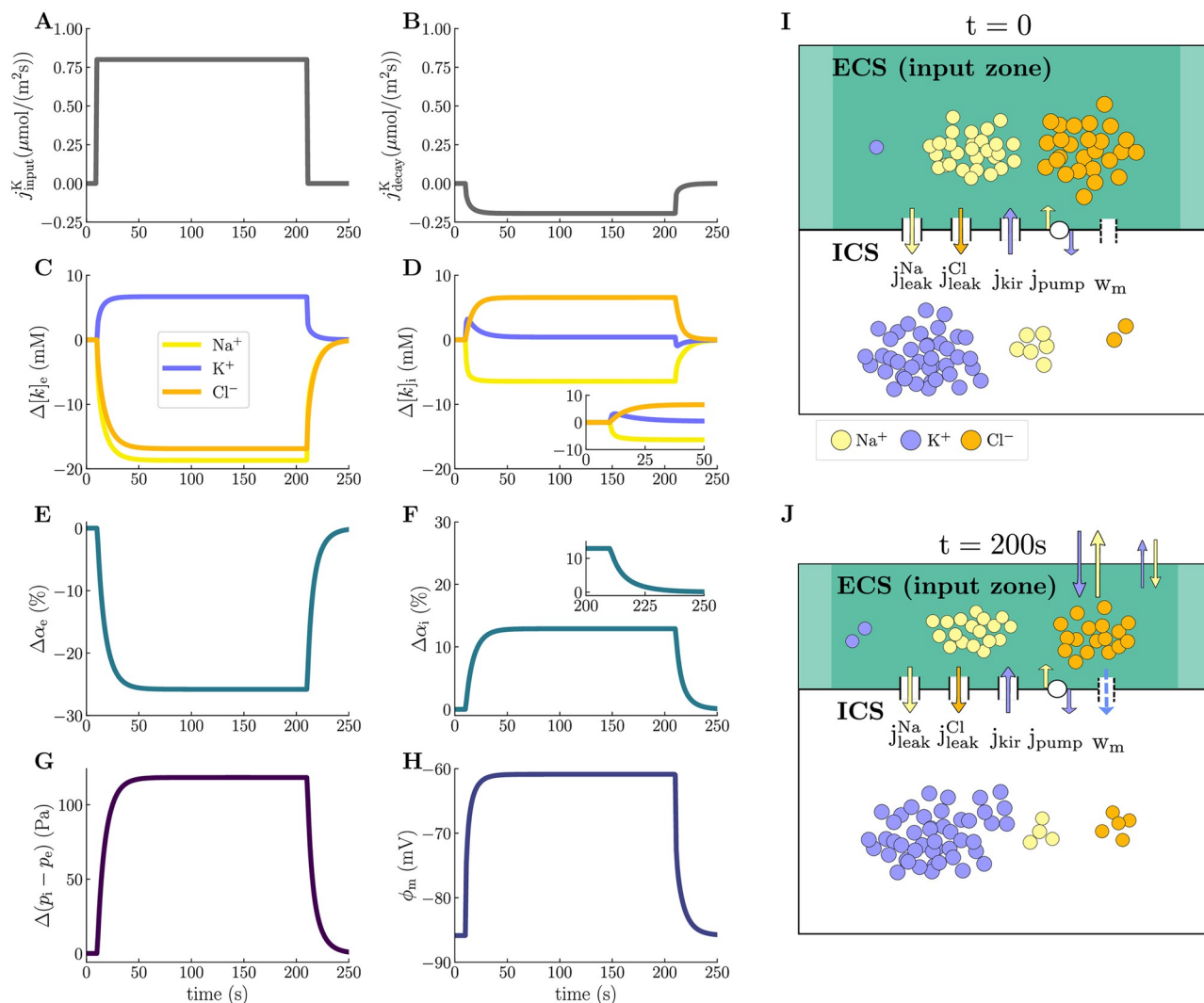
Fig 2. Electrical, chemical, and mechanical dynamics in the input zone during local neuronal activity. The panels display the time evolution of the \text{K}^+ -injection current (A) and \text{K}^+ -decay current (B), changes in the ECS (C) and ICS (D) ion concentrations, changes in the ECS (E) and ICS (F) volume fractions, changes in the transmembrane hydrostatic pressure difference (G), and membrane potential (H) at x = 150 \mu\text{m} (center of the input zone). All changes are calculated from baseline values, which are listed in Methods . Panel I and J display a schematic overview of ionic dynamics and swelling at respectively t = 0 s and t = 200 s at x = 150 \mu\text{m} .
