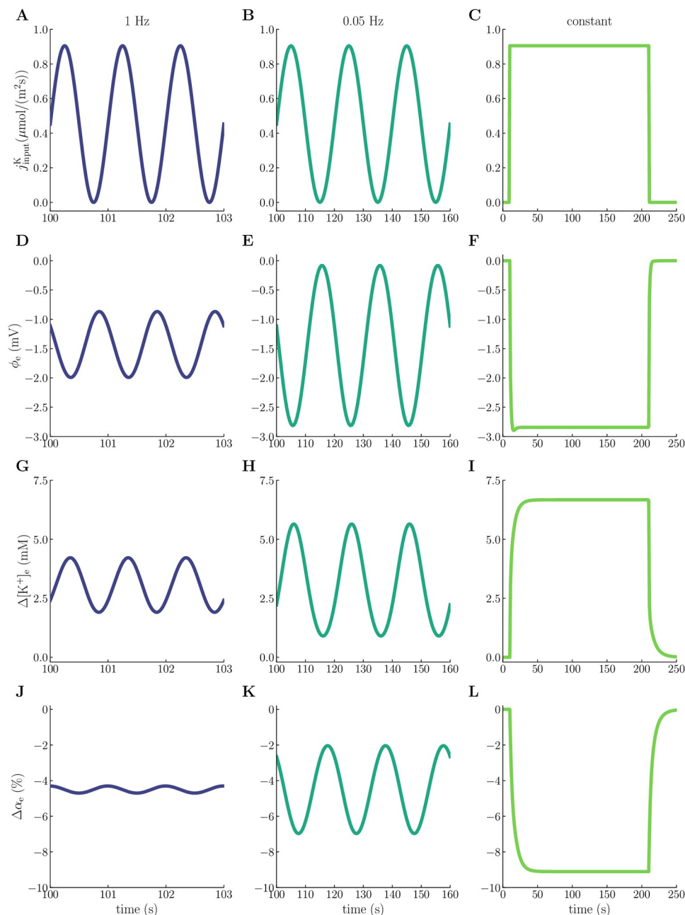
Fig 7. Electrical, chemical, and mechanical dynamics during slow, ultraslow, and constant stimuli. The panels display the time evolution of the K^+ -input current (A,B,C), extracellular potential (D,E,F), changes in the ECS K^+ concentration (G,H,I), and changes in the ECS volume fraction (J,K,L), at x = 150 \mu m (center of the input zone) for input varying at 1 Hz (left column), input varying at 0.05 Hz (middle column), and constant input (right column) (see Methods for details). All simulations correspond to model scenario M3.
