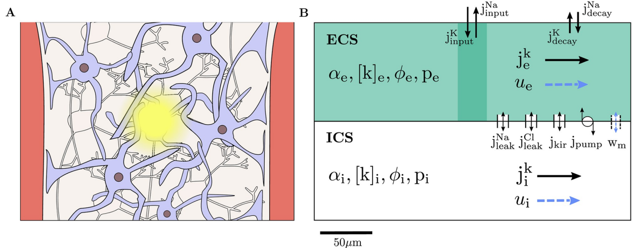
Fig 1. Model schematics. Illustration of brain tissue between two blood vessels with astrocytes (purple), neurons (grey), and ECS with neural activity in the center (A). The tissue is represented as a 1D domain of length 300\ \mu\text{m} including ICS (astrocytes) and the ECS (B). Within each compartment, the model describes the dynamics of the volume fraction ( \alpha ), the \text{Na}^+ , \text{K}^+ , and \text{Cl}^- concentrations ( [\text{Na}^+] , [\text{K}^+] , [\text{Cl}^-] ), the electrical potential ( \phi ), and the hydrostatic pressure ( p ). Neuronal activity is implicitly represented by \text{K}^+ and \text{Na}^+ input currents ( j_{\text{input}}^{\text{K}} and j_{\text{input}}^{\text{Na}} ) and decay currents ( j_{\text{decay}}^{\text{K}} and j_{\text{decay}}^{\text{Na}} ) across the whole domain. Transmembrane currents include an inward rectifying \text{K}^+ current ( j_{\text{kir}} ), \text{Na}^+ and \text{Cl}^- leak currents ( j_{\text{leak}}^{\text{K}} and j_{\text{leak}}^{\text{Cl}} ), and a \text{Na}^+/\text{K}^+ pump current ( j_{\text{pump}} ). Intra- and extracellular currents ( j_i^k and j_e^k ) are driven by electrodiffusion and advection. Fluid can travel across the membrane ( w_m ) and compartmentally in the intra- and extracellular space ( u_i and u_e ).
