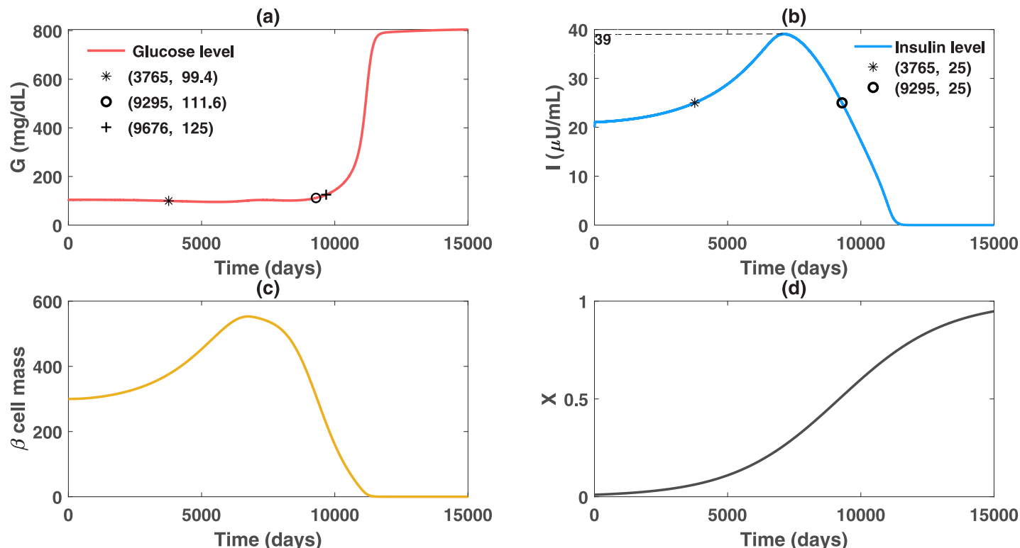
Fig 6. Dynamics of glucose, insulin and functional beta-cell mass for patient B with severe obesity ( X approaches 1 progressively). Patient B is assumed to have a lower insulin resistance level and less beta-cell hyperresponsiveness to the obesity-related factor than patient A does. Graph (b) shows the hyperinsulinemic stage of patient B lasts for 15.2 years, which is 3.3 years shorter than patient A does in Fig 2. The maximal insulin level he would develop is 39 \mu\text{U}/\text{ml} , which is 27.6 \mu\text{U}/\text{ml} lower than the highest level that patient A attains. During this hyperinsulinemic stage, the glucose levels can be well controlled beneath 111.6 \text{ mg}/\text{dl} . Additionally, patient B would not step into the diabetic stage until day 9676, which is 11.5 years later than patient A does.
