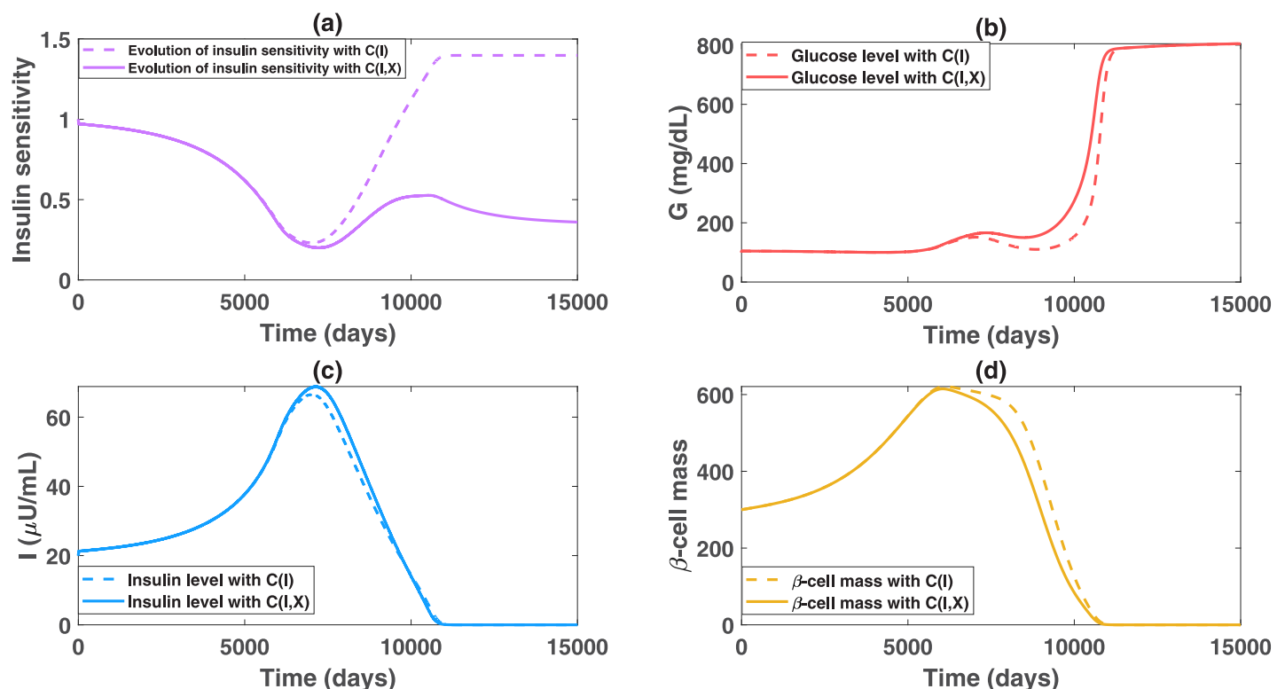
Fig 3. Comparison of the insulin sensitivity and G\beta dynamics using C(I) and C(I, X) in the model. The function C(I, X) is chosen to be C(I) \cdot \left(1 - \frac{0.8X^4}{X^4 + 0.5^4}\right) , where C(I) is given in model (1). The other parameters maintain the same as in Fig 2. Graph (a) shows the time evolution of the insulin sensitivity C(I) in the dashed curve and C(I, X) in the solid curve. Graphs (b), (c), and (d) exhibit the corresponding G\beta dynamics under the two insulin sensitivity functions.
