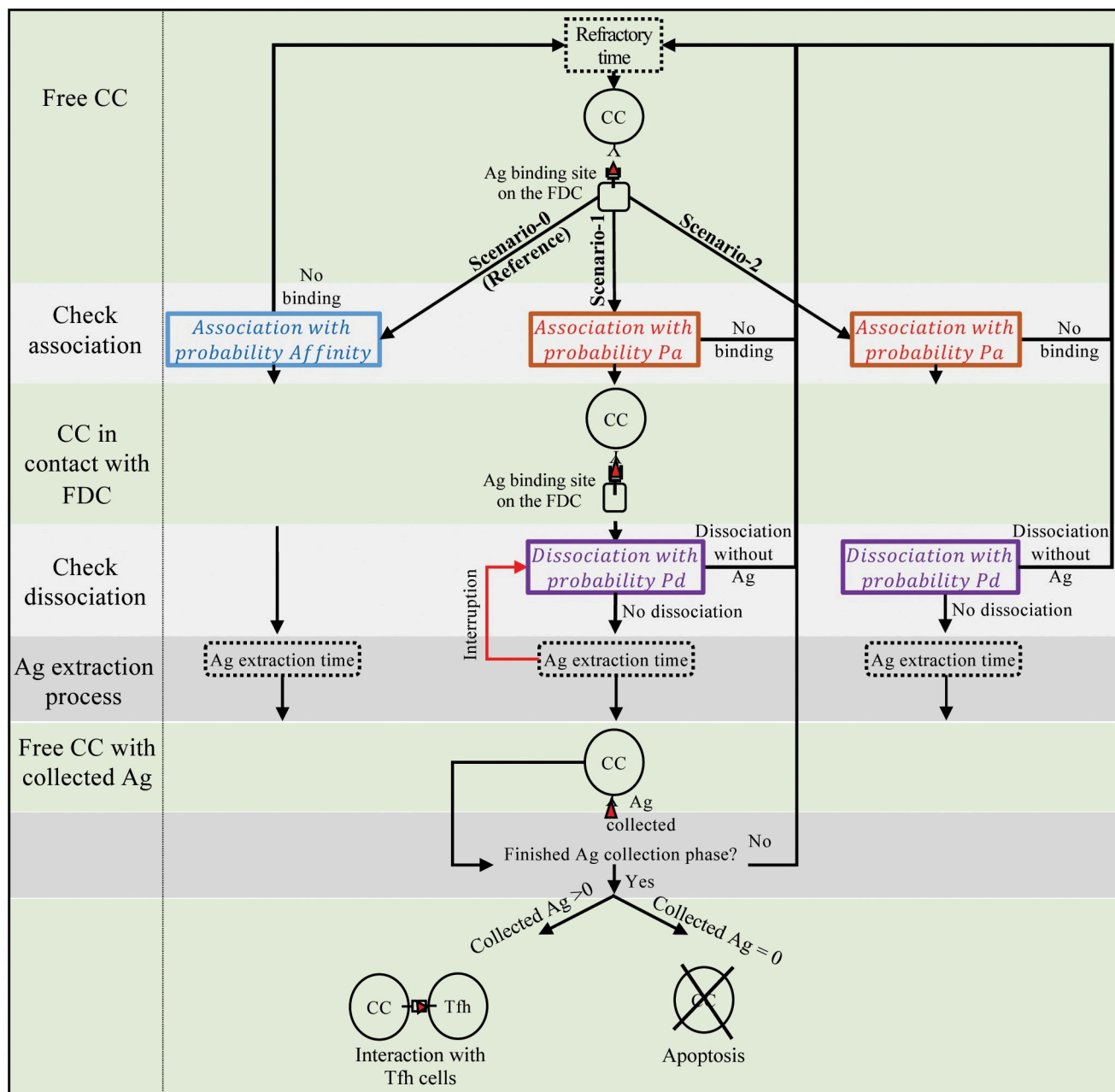
Fig 2. Schematic of Ag collection scenarios. Three mechanisms of Ag collection based on affinity and kinetic selection. The green rows denote the steps that the scenarios have in common. The starting point of each scenario is the event at which a free CC arrives at an Ag binding site. All scenarios end when the Ag collection phase is finished (last grey row), and the cell can engage in T-cell interactions. When no Ag is collected within 42 minutes, the CC will go into apoptosis. (A) Scenario-0: Competition for Ag depends on affinity directly. The CC's probability of binding to Ag depends on the local Ag concentration (not shown in the figure) and CC's affinity. After binding, the Ag extraction always starts directly. CC stays in bond until the Ag extraction process is finished after a period specified by a parameter 'Ag extraction time' whereafter the CC captures the Ag. Subsequently, the CC may collect more Ag or engage in T-cell interactions. (B) Scenario-1: Competition for Ag collection depends on association ( P_a ) and dissociation ( P_d ) probabilities of CC that rely on the affinity. In this scenario, a CC associates to Ags presented on FDCs according to Ag concentration at the binding site and P_a . In the next time step, the bond dissociates with a probability of dissociation ( P_d ) or otherwise, CC initiates the Ag extraction process. During the Ag extraction process, the bond between CC and Ag still can get disrupted probabilistically (red arrow) at each time-step ( dt = 0.002 h) with probability P_d that may lead to disruption of Ag extraction before it is fully complete, in which case the CC dissociates without obtaining Ag. Subsequently, if the bond between CC and Ag does not dissociate due to interruptions during the Ag extraction, CC collects the Ag and re-engages in another interaction. (C) Scenario-2: Similar to Scenario-1, only there are no interruptions after initiation of Ag extraction.
