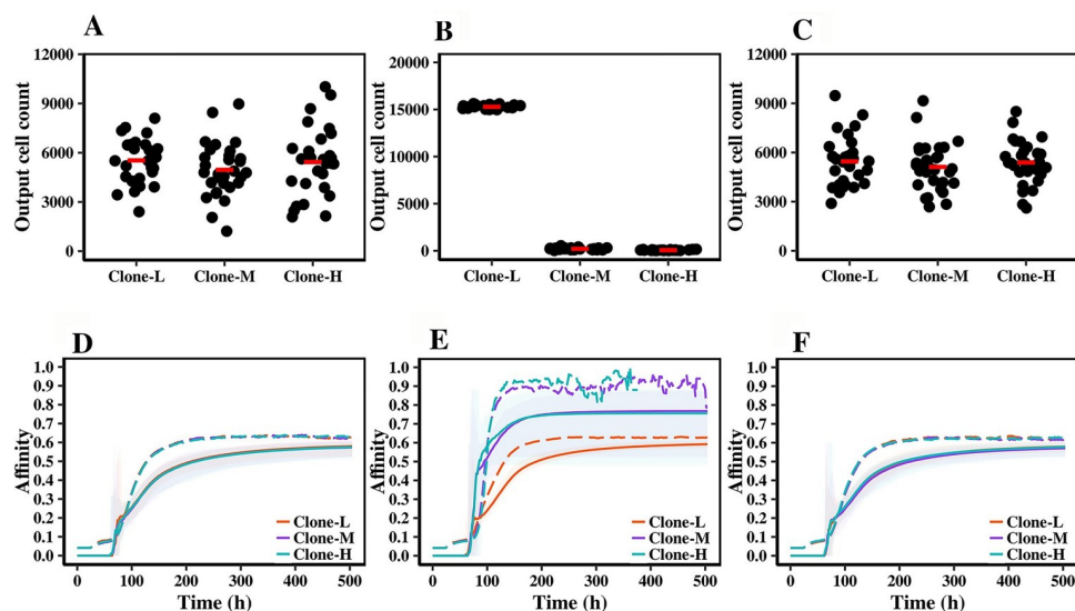
Fig 4. OCs production and affinity maturation. Results are obtained from 30 simulations. (A), (B) and (C) represent produced OCs from each clone in the reference scenario, Scenario-1 and Scenario-2, respectively. Each dot represents OCs produced in a single simulation. Red lines denote the average. (D), (E) and (F) represent the average affinity of living GC B cells (dashed lines) and the cumulative average of produced OCs (solid lines) belonging to each clone in the reference scenario, Scenario-1 and Scenario-2, respectively. Shaded areas indicate the maximum and minimum of OC's average affinity in 30 simulations.
