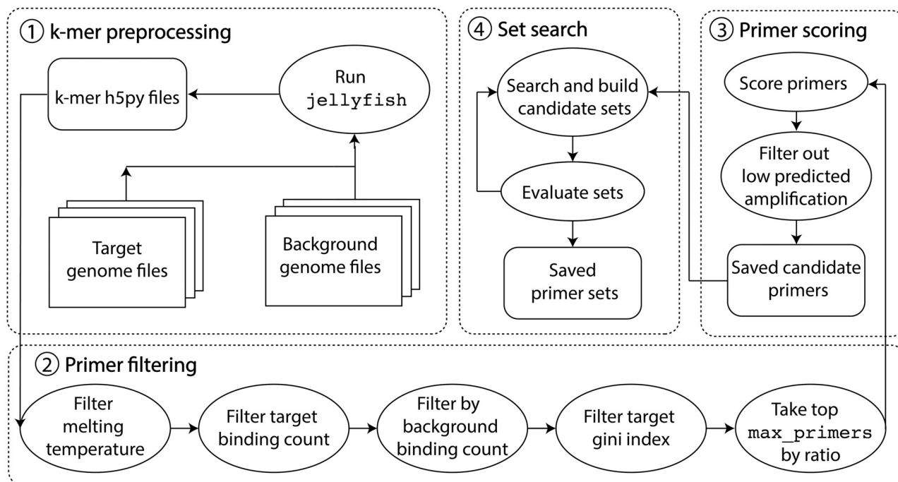
Fig 1. Overview of the swga2.0 pipeline. The process is broken into four stages: 1) preprocessing of locations in the target and off-target genomes, 2) filtering motifs in the target genome based on individual primer properties and frequencies in the genomes, 3) scoring the remaining primers for amplification efficacy using a machine learning model, and 4) searching and evaluating aggregations of primers as candidate primer sets.
