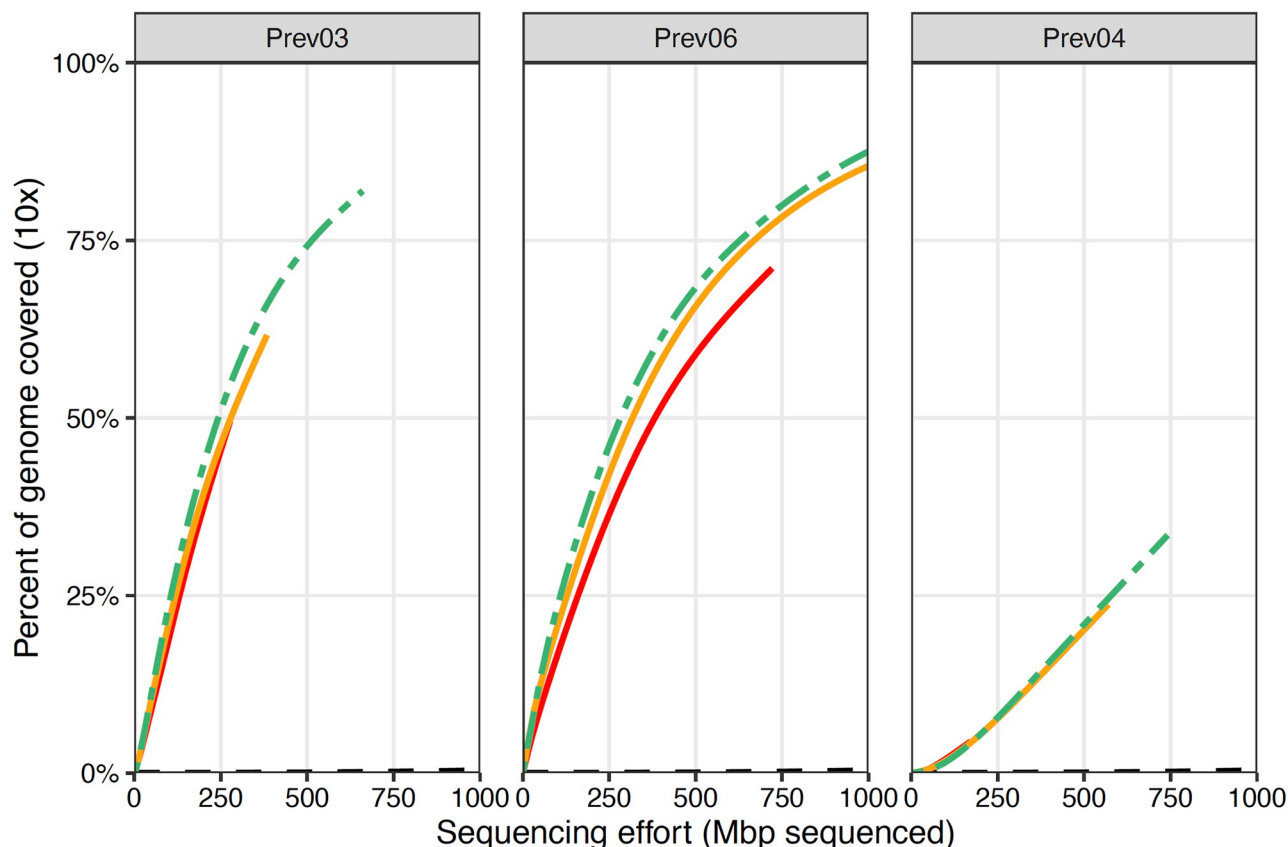
Fig 6. Deeper sequencing of the three successful primer sets—Prev03, Prev06, and Prev04—confirms the efficient and even selective amplification of P. melaninogenica . The solid colored lines indicate individual replicates and the green dashed line represents the pooled total. Each of the three primer sets yield dramatic increases in sequencing depth compared to the unamplified samples (black dashed line). Each primer set reached 10× coverage across 23–74% of the target genome, while the unamplified samples reached 10× coverage at <1% of the target genome, with 500 Mbp of sequencing effort.
