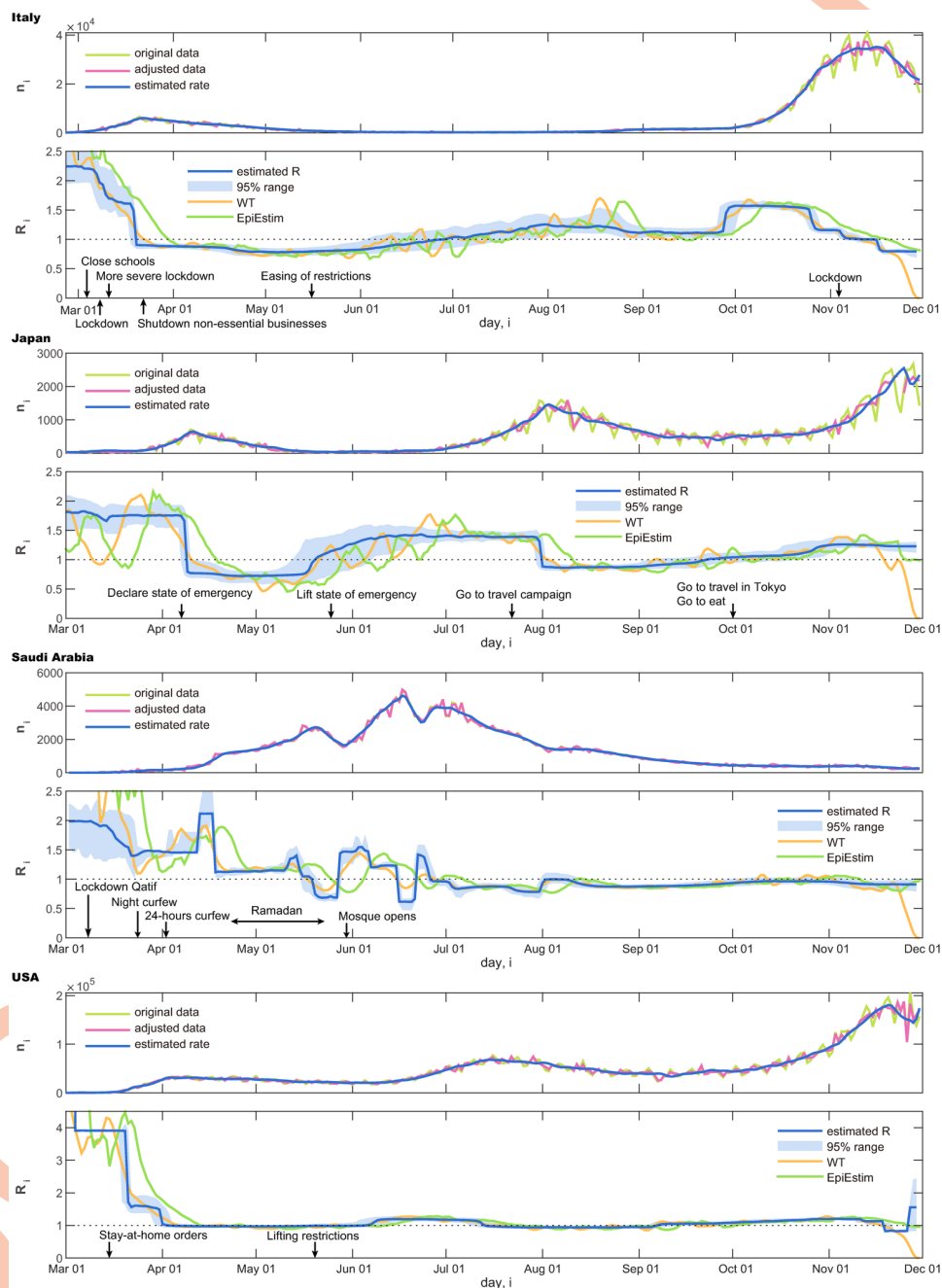
Fig 5. Number of daily new cases and the reproduction number \hat{R}_t estimated using the state-space method. Italy, Japan, Saudi Arabia, and the USA.
