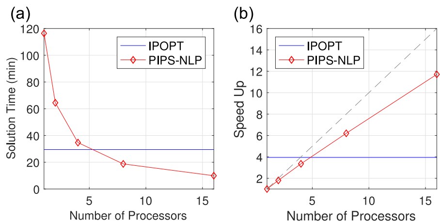
Fig 12. Performance comparison of general solver Ipopt and the structure-exploiting solver PIPS-NLP (P1-P2, Model 1). (a) Solution time for P2 using Ipopt and PIPS-NLP . The y-axis shows the solution time and the x-axis shows the number of cores used. For Ipopt the single core solution time is given by the horizontal blue line. (b) The y-axis represents the speed-up (the single-core solution time divided by the multi-core solution time). The blue line is the single-core solution time of PIPS-NLP divided by the single-core solution time of Ipopt . The grey dashed line represents the strong scaling line.
