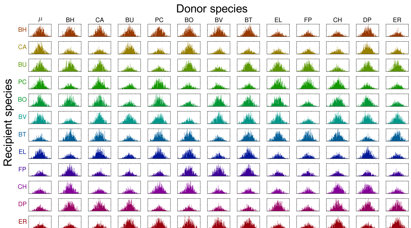
Fig 9. Posterior (marginal) densities for estimated parameters (P1, Model 1). Each subplot shows the histogram of the samples from the approximate parameter posterior. The x-axis represents the values of the estimated parameters and the y-axis represents the frequencies. The subplots on the first column show the distribution of the growth rates \mu_s and the rest of the subplots show distributions of the interaction parameters \alpha_{sr} . Recipient and donor species are listed in rows and columns, respectively. The x-axis is scaled to show \mu \pm 3\sigma where the \mu is the mean and the \sigma is the standard deviation of the posterior distribution.
