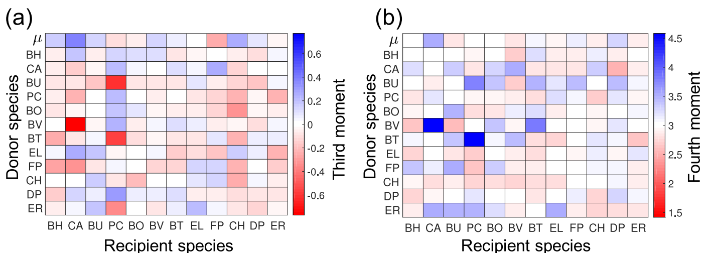
Fig 11. Third and fourth momentum of posterior (P1, Model 1). (a) Heat map presents the third momentum of the parameter posterior density (normalized by \sigma^3 ). (b) The heat map represents the fourth momentum of the posterior density (normalized by \sigma^4 ). (a-b) The first row shows the standard deviations of the growth rate parameters \mu_s and the rest of the rows show the standard deviations of the interaction coefficients \alpha_{ss'} . Recipient and donor species are on the x and y-axis, respectively.
