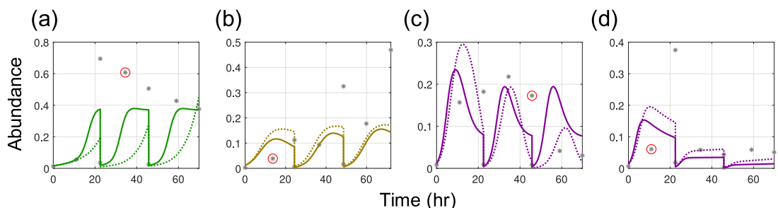
Fig 6. Improvement of model fitting by using CVaR ( k -max) MAP formulation (P1, Model 1). Model fits for 4 experiments selected among the experiments with 10 largest prediction errors (1/2)(\eta_{k,s}(t) - \bar{\eta}_{k,s}(t))^2 / \sigma_{k,s}(t)^2 . The model fits from standard MAP formulation (dotted line) are compared with the model fits from CVaR formulation with \beta = 0.9 (solid line). (a) gLV model fits to pairwise community experiment of PC in the presence of EL. (b) gLV model fits to pairwise community experiment of CA in the presence of ER. (c) gLV model fits to pairwise community experiment with CH in the presence of PC. (d) gLV model fits to pairwise community experiment with CH in the presence of BO.
