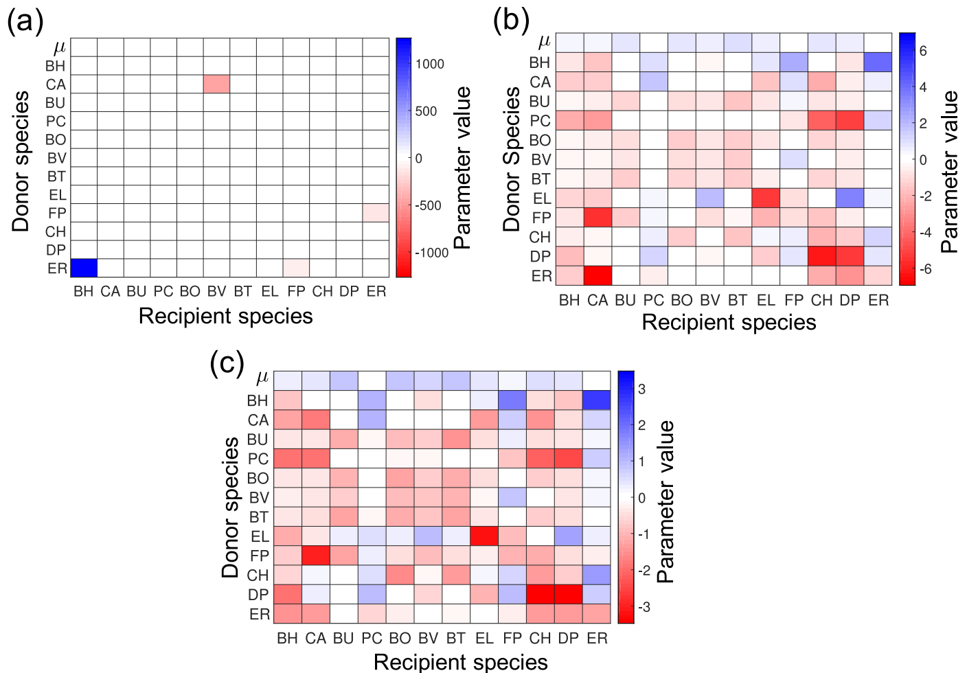
Fig 3. Parameter estimates with MAP formulations (P1, Model 1). (a) Estimates using MAP formulation with no prior information. (b) Estimates using L1 prior. (c) Estimates using L2 prior. (a-c) The first row shows values for the growth rate parameters \mu_s and the rest of the rows show values for the interaction parameters \alpha_{ss'} . The species name corresponding to s and s' are presented on the x and y axes. Recipient and donor species are on the x and y -axis, respectively.
