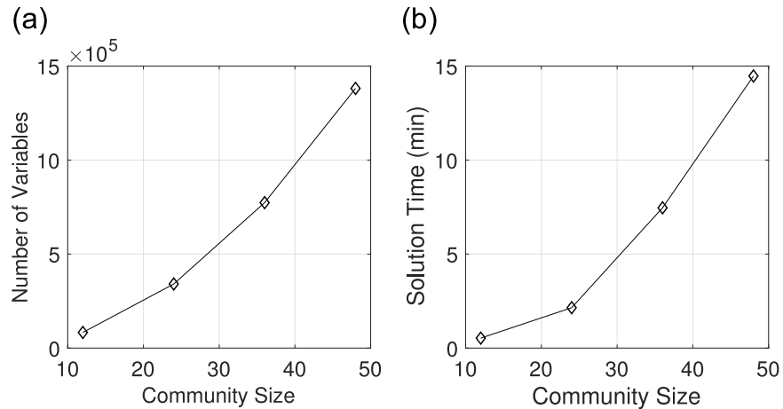
Fig 13. Computational scalability with larger communities (S1-S4, Model 1). (a) Number of variables against community size (total number of species). (b) The computation times for problems S1-S4 (see Table 2). The problems were solved with PIPS-NLP on 12 parallel cores (Intel(R) Xeon(R) CPU E5-2698 v3 processor running at 2.30GHz).
