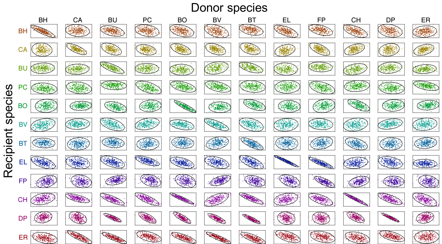
Fig 10. Correlations between parameter pairs (P1, Model 1). Each subplot shows the 95% confidence regions (solid ellipses) of the approximate parameter posterior distributions and the sample points (dots). The subplots on the s -th row and s' -th column show the correlation of \mu_s and \alpha_{ss'} . Recipient and donor species are listed in rows and columns, respectively. Only a representative subset of parameter pairs is presented (there are a total 12,090 pairs).
