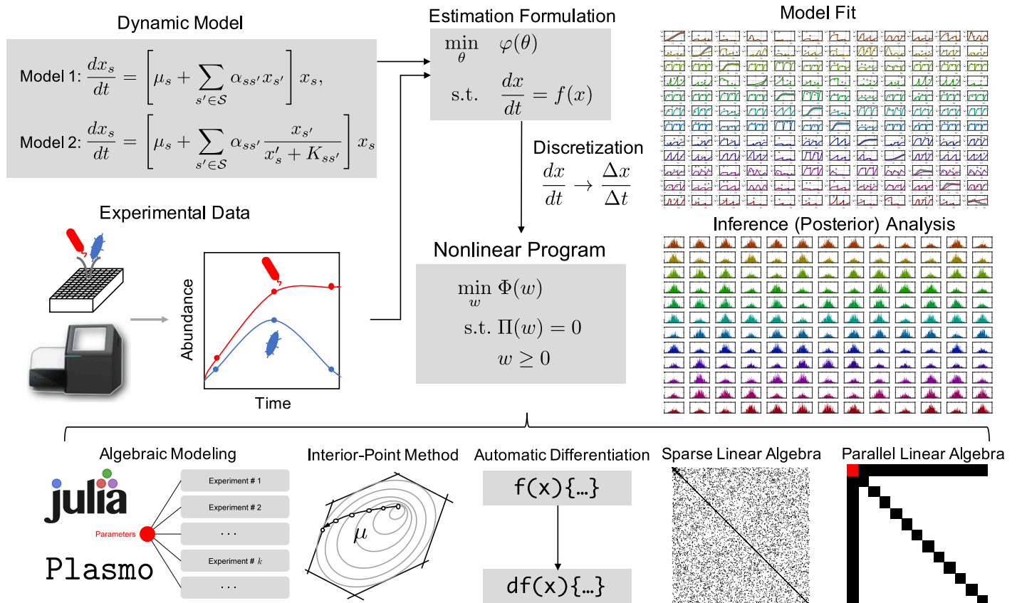
Fig 1. Illustration of the proposed estimation framework. Mathematical models for biological systems are often expressed as systems of differential equations with parameters that need to be estimated from experimental data. We formulate the estimation problem using a maximum a posteriori (MAP) formulation. This yields optimization problems constrained by differential equations that are transformed into fully algebraic nonlinear programs by using discretization schemes. The resulting NLPs can be easily implemented in algebraic modeling languages such as JuMP and PlasmO.jl that compute derivatives automatically and that are interfaced to powerful interior-point optimization solvers that exploit sparsity and structure to achieve high computational efficiency. The proposed framework is scalable, robust, easy-to-use, and flexible. These capabilities facilitate high-level tasks such as identification of parameter observability/uniqueness issues, model selection, and uncertainty quantification.
