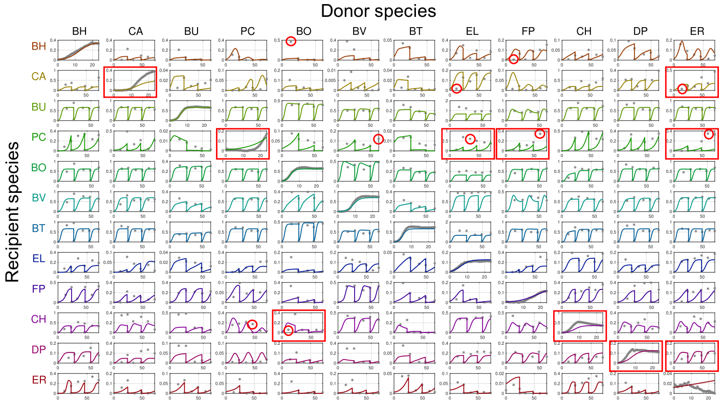
Fig 4. Fitting of experimental data (P1, Model 1). Subplots show the measured and predicted species abundance in the microbial community. The subplots on the diagonal show fitting for mono-species experiments. Subplots on the i -th row and j -th column shows fitting for the corresponding pairwise culture (the abundance of species i in the presence of species j ). Recipient and donor species are listed in rows and columns, respectively. For each subplot, the y -axis represents the absolute abundance in the community based on relative abundance multiplied by total biomass (OD600) and the x -axis represents the experiment time in hours. Data points are denoted by grey dots and dynamic model trajectories are denoted by solid lines. The data points highlighted with red circles are data points corresponding to the ten largest errors (1/2)(\eta_{k,s}(t) - \bar{\eta}_{k,s}(t))^2 / \sigma_{k,s}(t)^2 . The subplots highlighted with red boxes are subplots for the experiments with the ten largest total prediction errors \sum_{t \in \mathcal{T}_k} (1/2)(\eta_{k,s}(t) - \bar{\eta}_{k,s}(t))^2 / \sigma_{k,s}(t)^2 .
