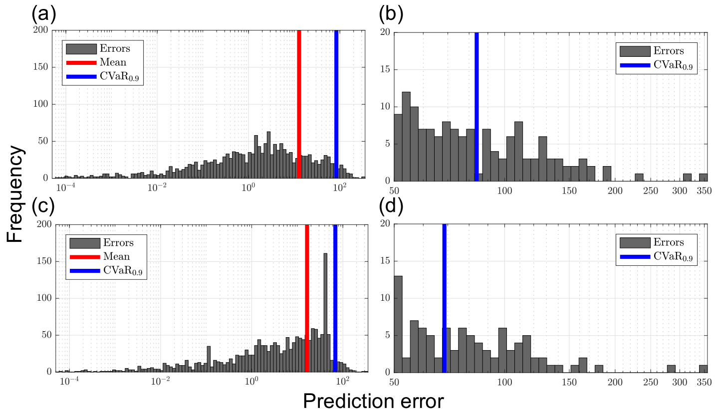
Fig 7. Histograms of fitting errors (P1, Model 1). (a) Error histogram for the standard MAP formulation. (b) Tail region of (a). (c) Error histogram for CVaR formulation. (d) Tail region of (c). (a-d) The x -axis represents the value of prediction error evaluated at the solution and the y -axis represents the frequency. The red and blue line represent quantiles: the overall mean of prediction errors (red) and the mean of largest 10% errors (blue).
