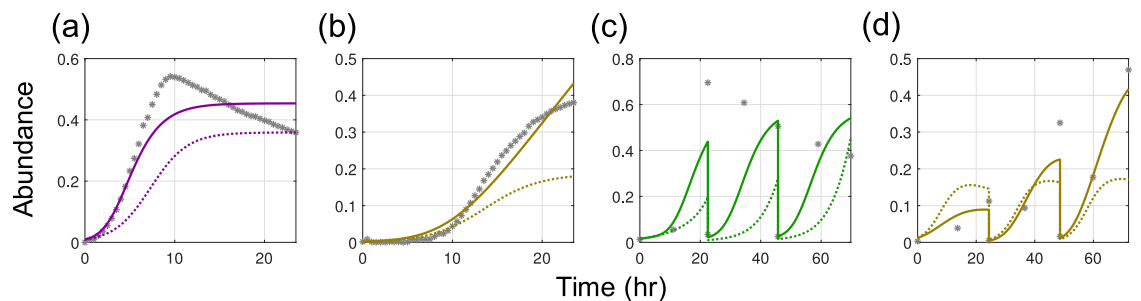
Fig 5. Improvement of model fitting with saturable gLV model (P1, Model 2). Model fitting for 4 experiments selected among the experiments with 10 largest total prediction errors. The gLV model fits (dotted line) are compared with those of the saturable model (solid line). (a) Model fits to monospecies experiment with CH. (b) Model fits to monospecies experiment with CA. (c) Model fits to pairwise community experiment with PC in the presence of EL. (d) Model fits for pairwise community experiment with CA in the presence of ER.
