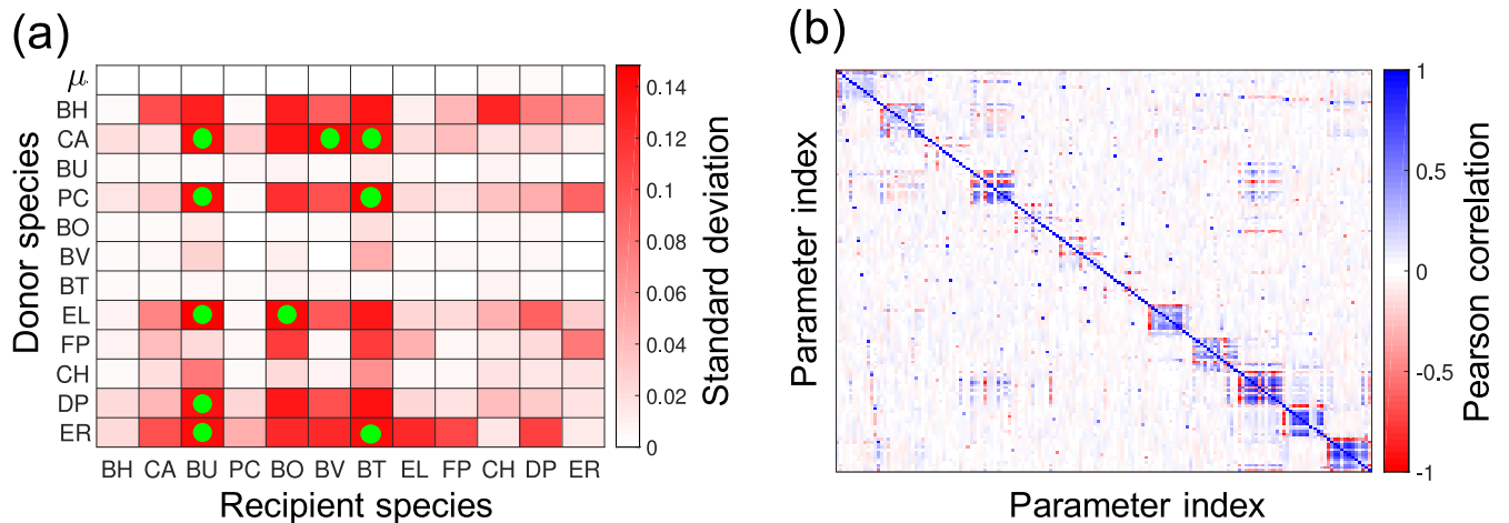
Fig 8. Parameter uncertainty and correlations (P1, Model 1). (a) Heat map presents the standard deviation for the parameter posterior density. The first row shows the standard deviations of the growth rate parameters \mu_s and the rest of the rows show the standard deviations of the interaction coefficients \alpha_{sr} . Recipient and donor species are on the x and y-axis, respectively. The data points highlighted with green circles are data points corresponding to the ten largest standard deviations. (b) The heat map represents the Pearson correlation coefficients of the posterior distributions. The x-axis and the y-axis represents the index of parameters where the parameter vector is constructed as \theta = (\mu_1, \alpha_{11}, \dots, \alpha_{1S}, \dots, \mu_S, \alpha_{S1}, \dots, \alpha_{SS}) . The block on the i -th row and j -th column is the Pearson correlation between the i -th and j -th component of parameter vector \theta .
